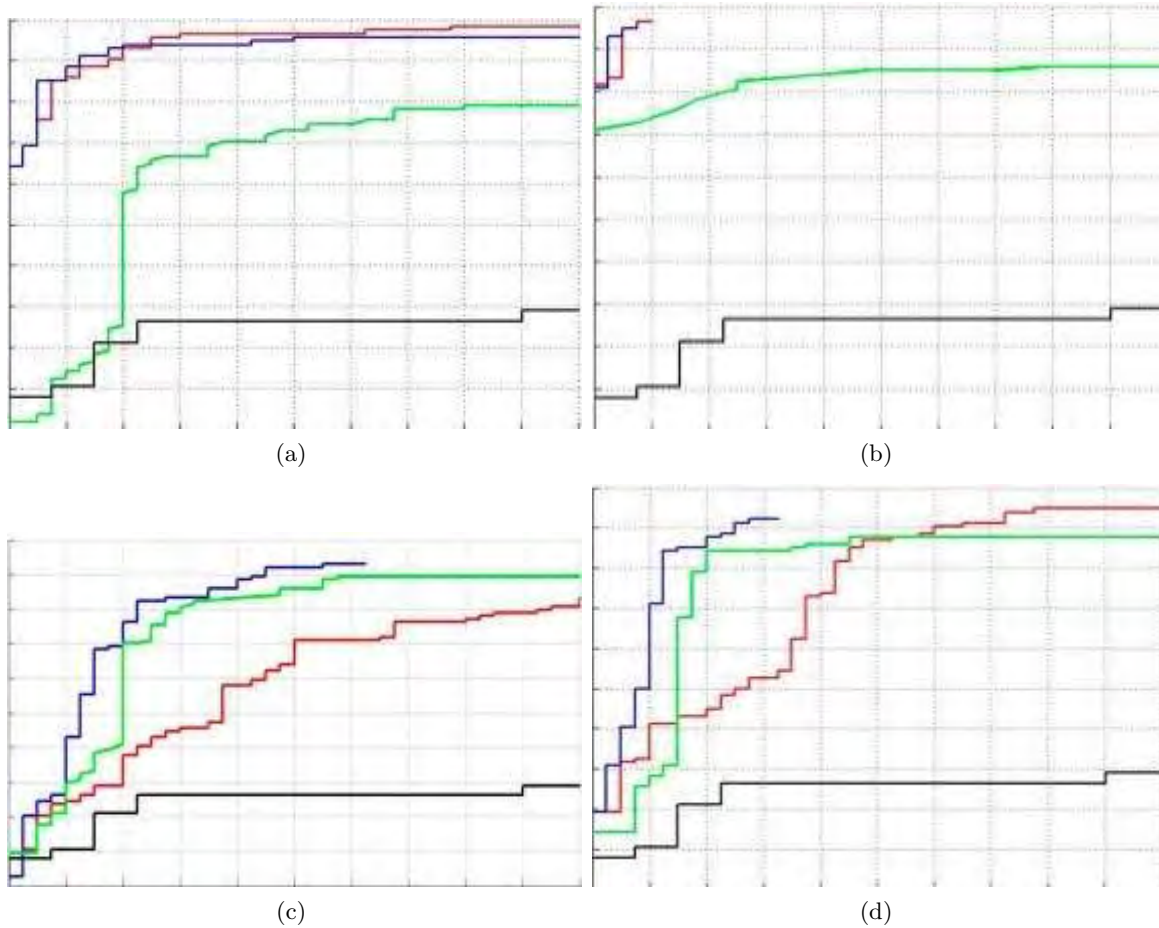
Figure 5. ROC Curves for each of the four GPR algorithms in which refilled holes were considered false alarms. Detection within a one meter halo of a refilled hole is considered a false alarm. In each of these plots, the red curve corresponds to the not cued GPR algorithm results, the blue curves corresponds to the cued GPR results, the black curve corresponds to the airborne alarm results and the green curve corresponds to the fused results (geometric mean of the features values) with the airborne alarms and the cued GPR alarms.
