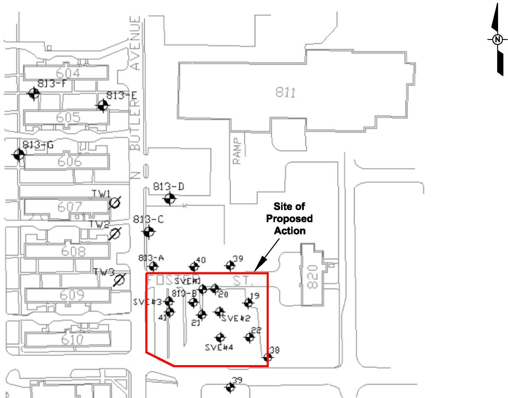
Figure 3-5 Proposed Site and ST-003 Location Maxwell Air Force Base - Gunter Annex, AL
