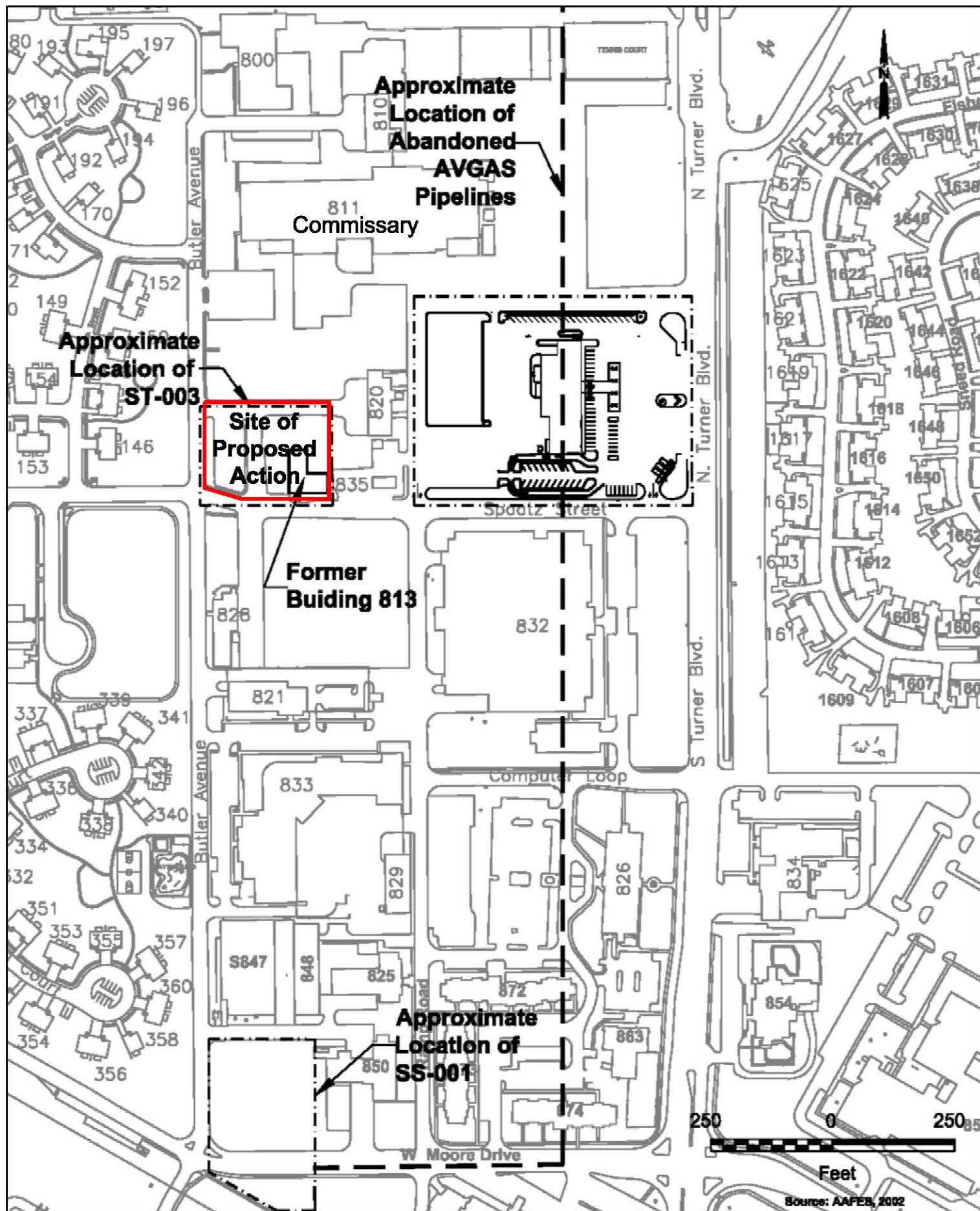
Figure 3-4 IRP Sites in Vicinity of Proposed Action Maxwell Air Force Base - Gunter Annex, AL
