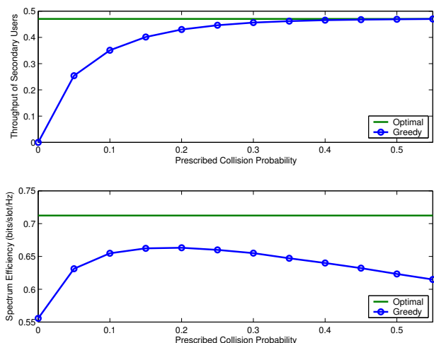
Fig. 3. OSA performance in the presence of sensing error ( N = 3 independent channels with the same bandwidth B = 1 and transition probabilities \{\alpha = 0.4, \beta = 0.5\} ).
