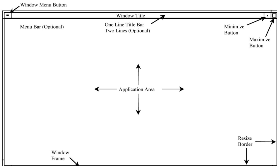
Figure 4.1. Window Layout.
