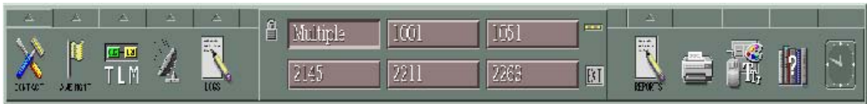
Figure 3.3. Toolbar Example.
