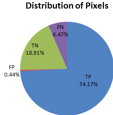
Figure 2.15: Pixel Distribution.
