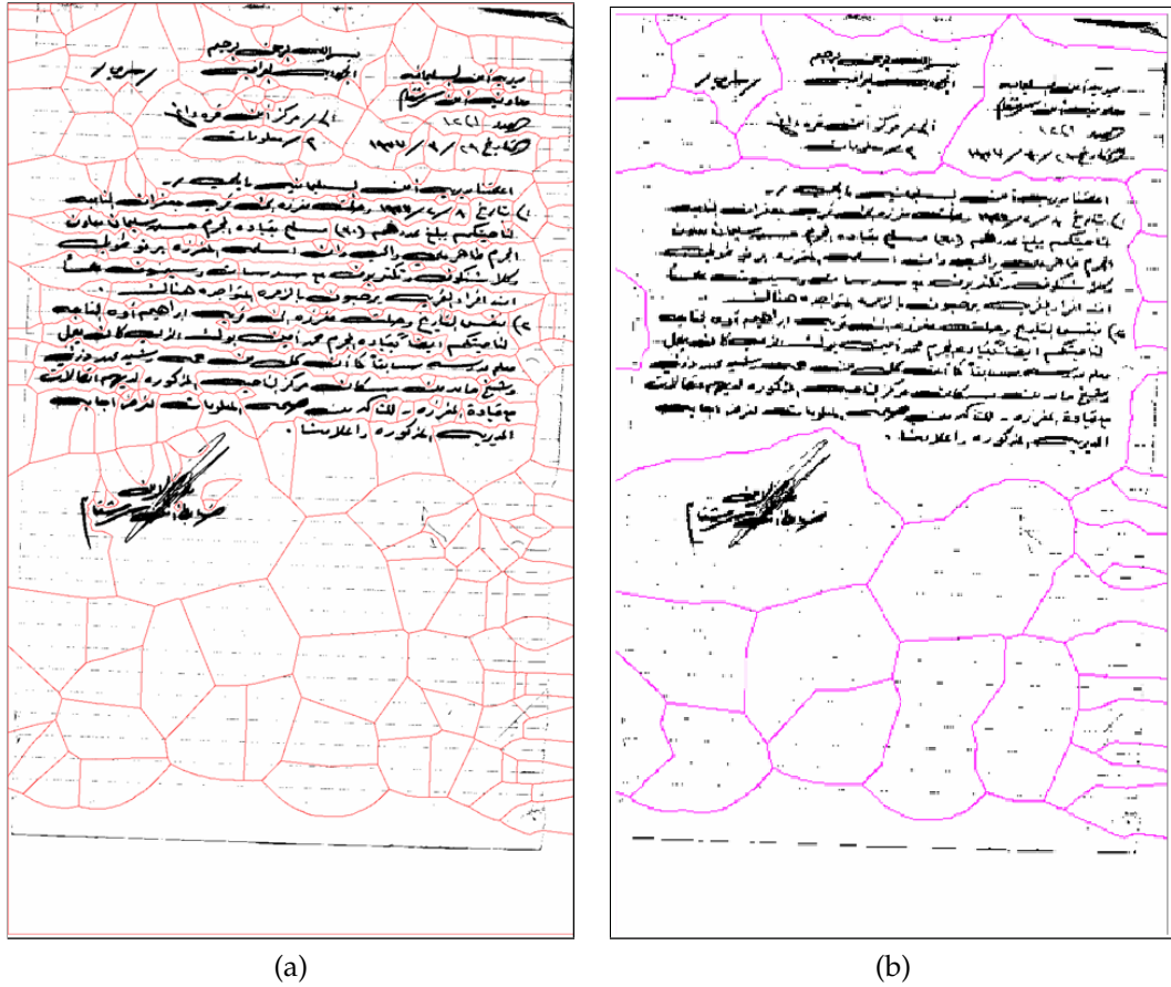
Figure 3.12: (a) Page Segmentation using the original Voronoi approach (b) Page Segmentation after finding word separation thresholding using the improved valley-finding algorithm.
