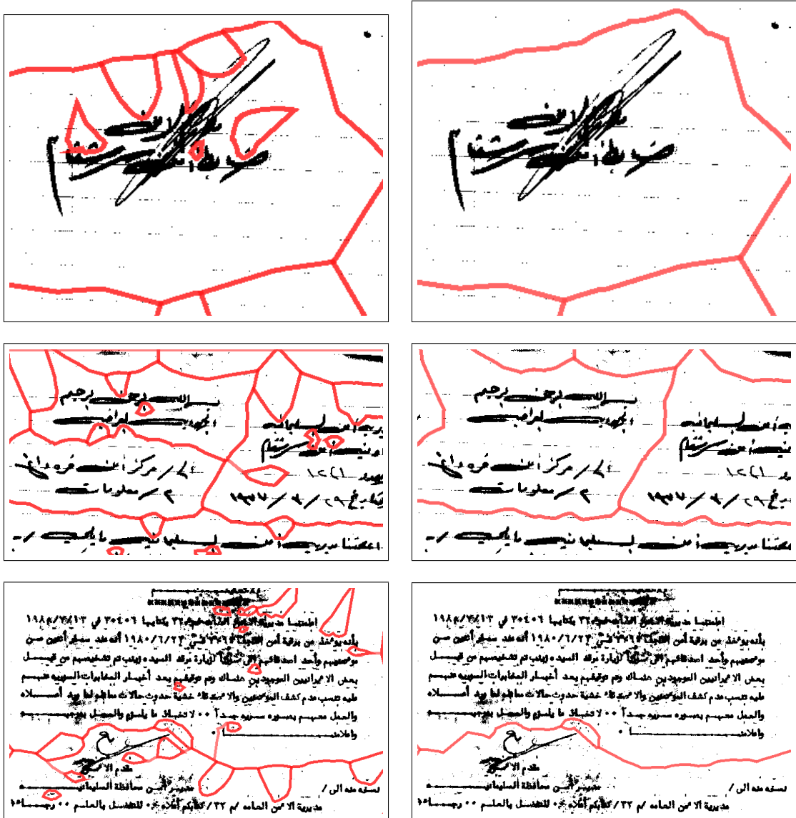
Figure 3.9: Illustration of results with and without NN associativity: The left side shows segmentation results without nearest-neighbor associativity and the right side shows the corresponding results with nearest-neighbor associativity.
