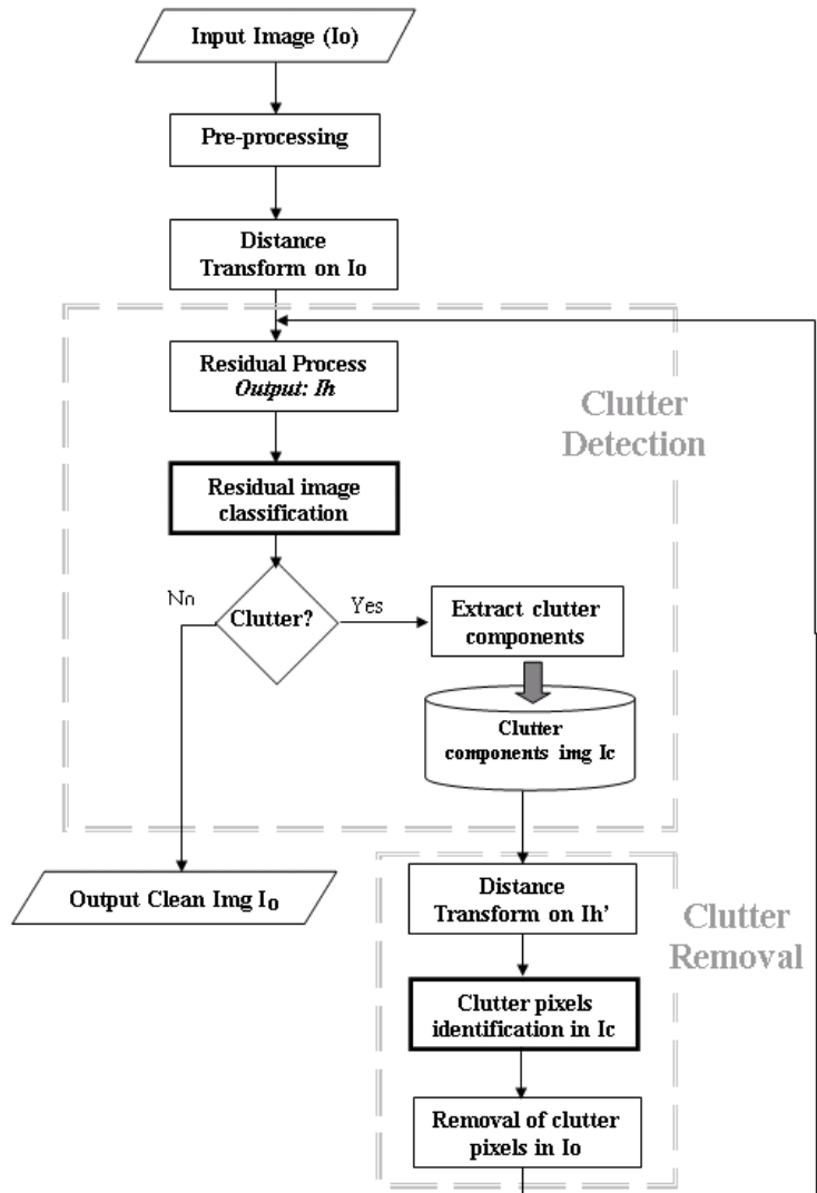
Figure 2.14: Clutter Detection and Removal.
