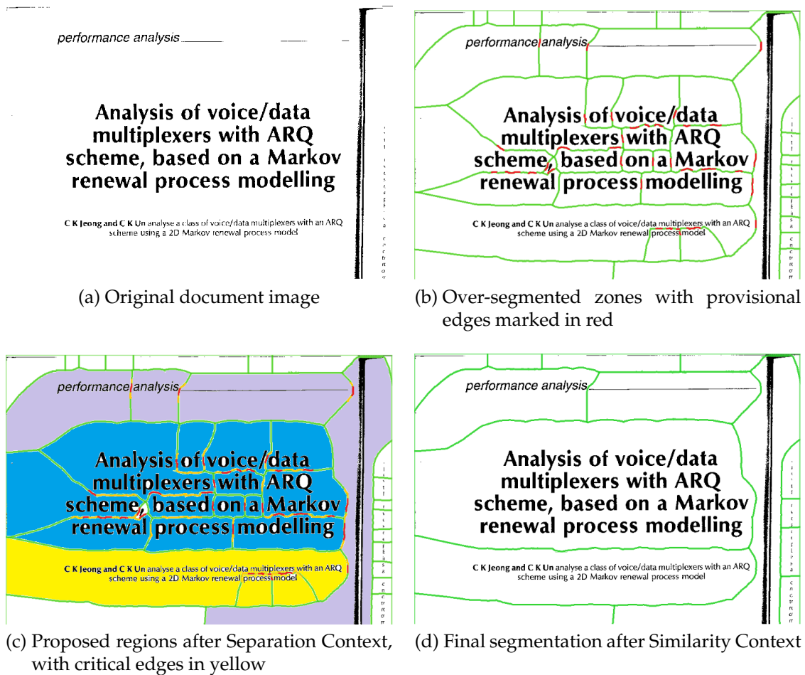
Figure 3.19: Context-aware phases of Voronoi++.
