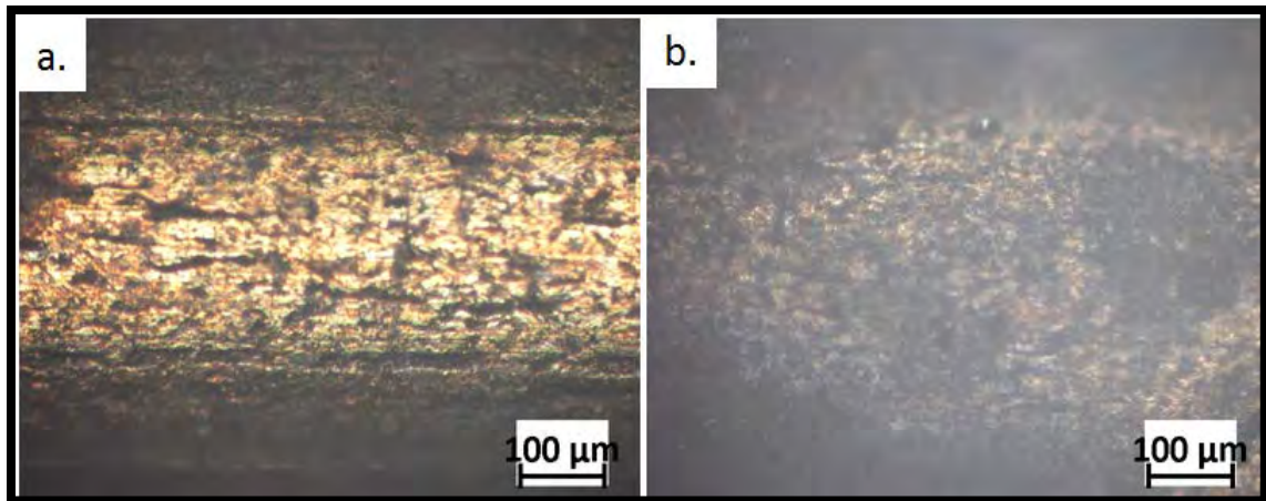
Figure 25. Optical images of the brass substrate in its longitudinal axis. Image (a.) is the as-is brass sample without surface preparation. Image (b.) is brass after the initial attempt to chrome coat. The post treated sample appears to have a layer of black particles.
