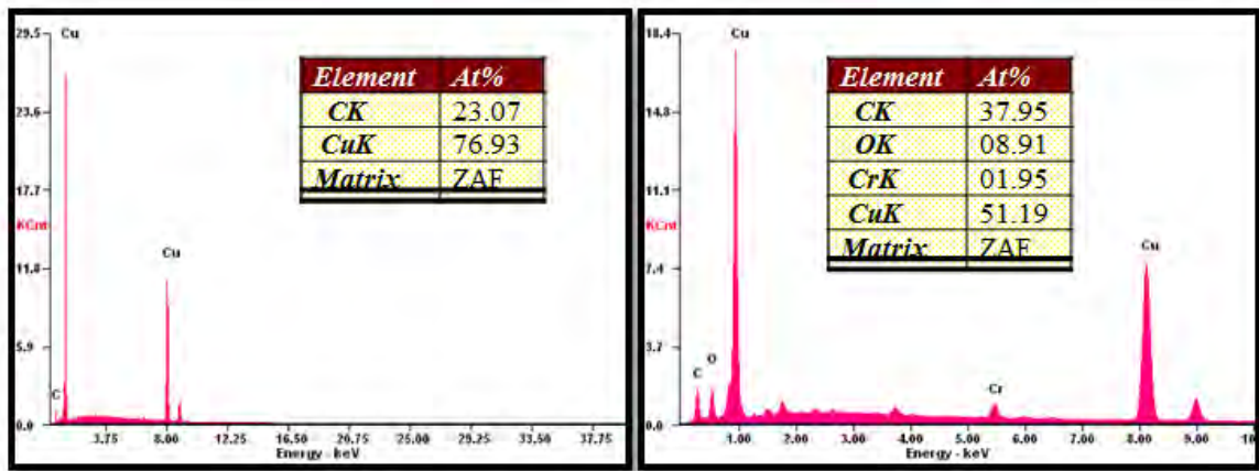
Figure 56. EDS analysis of the surface of the copper substrates. (a.) Sample 18 (1:2:1) contained less oxygen and carbon when compared to (b.) Sample 21 (1:3:1). Sample 21 also contained limited chromium deposits treatment.
