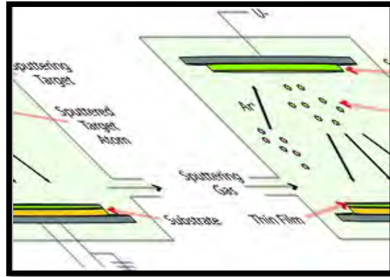
Figure 6. Sputtering deposition process, from [17].
