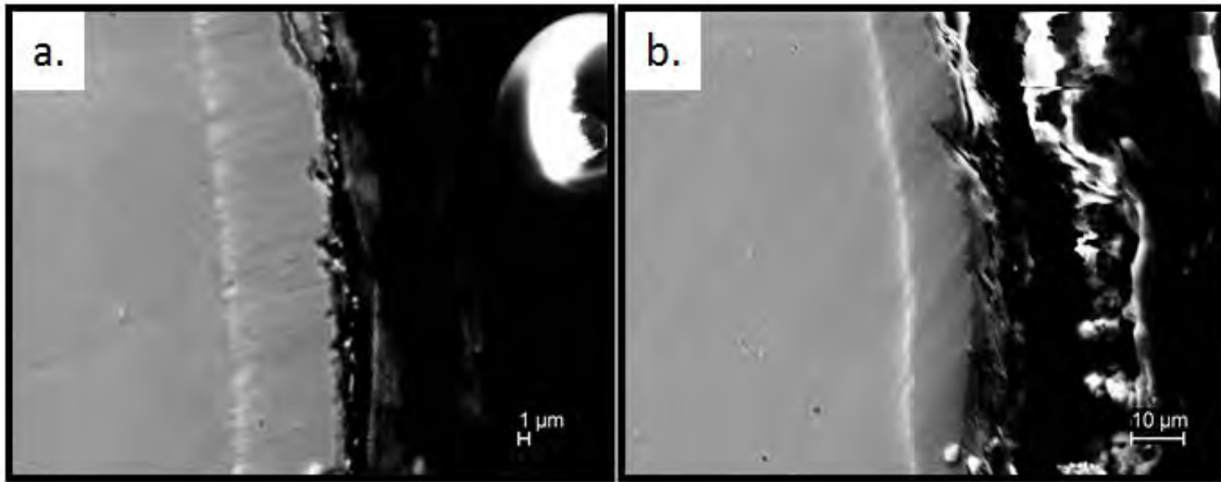
Figure 61. (a.) SEM micrographs of Sample 20 treated with a 1:2:1 coating mixture ratio to 850°C showed an outer layer on the surface. (b.) Sample 23 treated with a 1:3:1 coating mixture ratio to 1000°C showed an outer surface layer.
