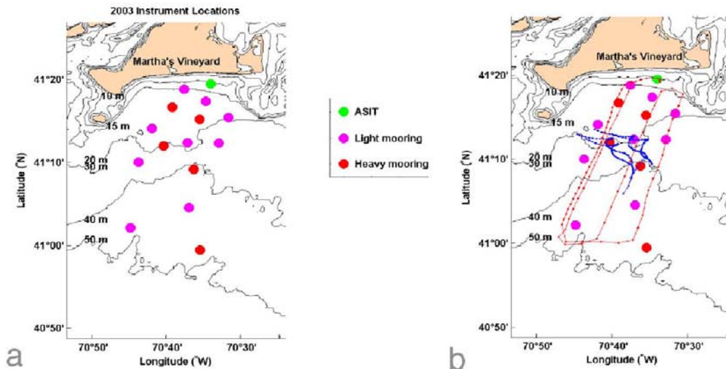
Figure 2. a) The locations south of Martha’s Vineyard of the 5 heavy surface moorings, 10 light moorings deployed in 2003 along with the location of the Air-Sea Interaction. b) Example tracks (blue) from one deployment of the drifting thermistor strings deployed during the IOP and of one deployment of the towed chain by FV Nobska (red) during the IOP to illustrate the additional sampling done over a wide range of spatial scales.
