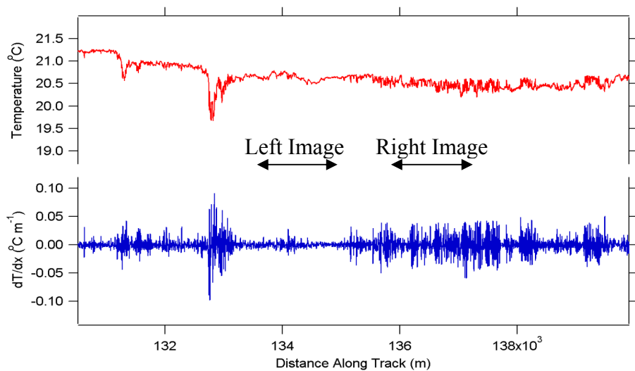
Figure 3. (a) Examples of fine-scale IR imagery as observed from the aircraft under very low wind speed. Each image is roughly 160 m x 200 m and the top of the images is West. (b) Temperature and its derivative measured along the flight track that correspond to the observations in (a).
