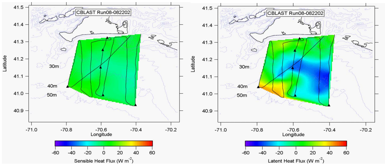
Figure 1. Maps of the sensible and latent heat flux variability determined using the sea surface temperature measurements produced using the low-noise data from the imager (in Point mode). The black trace is the Skymaster flight track.
