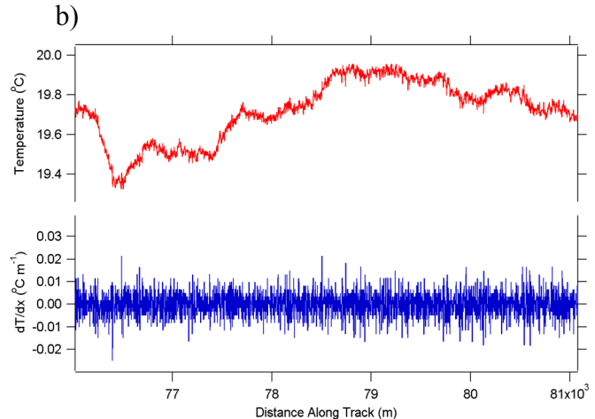
Figure 4. (a) Example of fine-scale IR imagery as observed from the aircraft under moderate wind speed. Each image is roughly 160 m x 200 m, the top of the images is East, and the wind is from the NE. (b) Temperature and its derivative measured along the flight track that correspond to the observations in (a).
