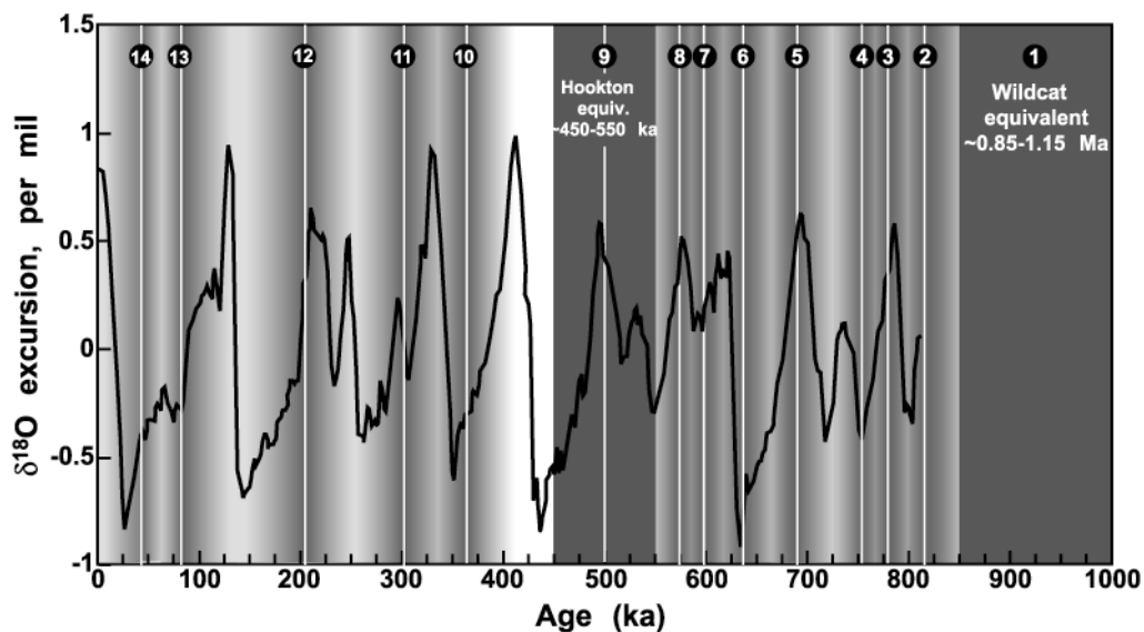
Figure 1 – Stacked \delta^{18}O curve derived from fourteen different benthic records globally (Medeiros et al., 2000). Vertical lines show estimated ages of Eel River Basin seismic unconformities; shading represents uncertainty in our age estimates. Solid gray areas represent estimated hiatus durations of the "Hookton" and "Wildcat" equivalents (Surfaces 1 and 9). Note the increased frequency of unconformity formation prior to ~550 ka, mimicking the obliquity-dominated 41 kyr glacioeustatic cycles during that same interval. After the Hookton Datum hiatus, the frequency of unconformity formation decreases, and coincides with the eccentricity-dominated 100 kyr cycles during that interval. The apparent correspondence between \delta^{18}O cyclicity and unconformity formation both before and after the orbitally-dominated transition implies that glacioeustasy controls formation of these surfaces, at least in part.
