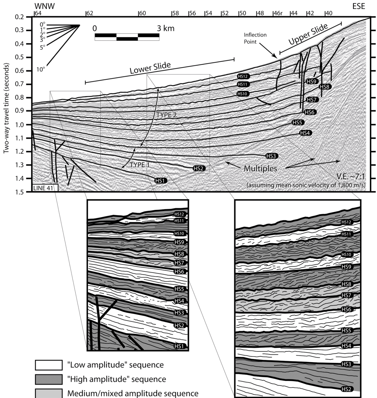
Figure 2. Dip seismic profile 41 showing sequences mapped through the axis of the Humboldt Slide (HS). Bold, steeply dipping lines represent faults. True dips are indicated at upper left. Inset figures from middle of the “lower slide” (right) and near the toe of the slide (left) indicate high-, low-, and mixed-amplitude sequences, as well as internal sequence geometries.
