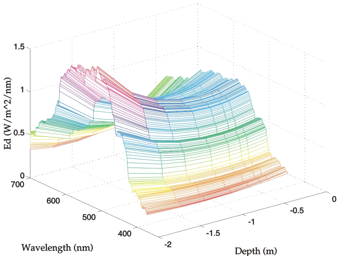
Figure 1. Downwelling irradiance over a seagrass bed surrounded by sand, 3 meters total water depth. Contrary to expectations, the light level increases with depth due to the contribution from internally reflected light from adjacent, sandy bottom.
