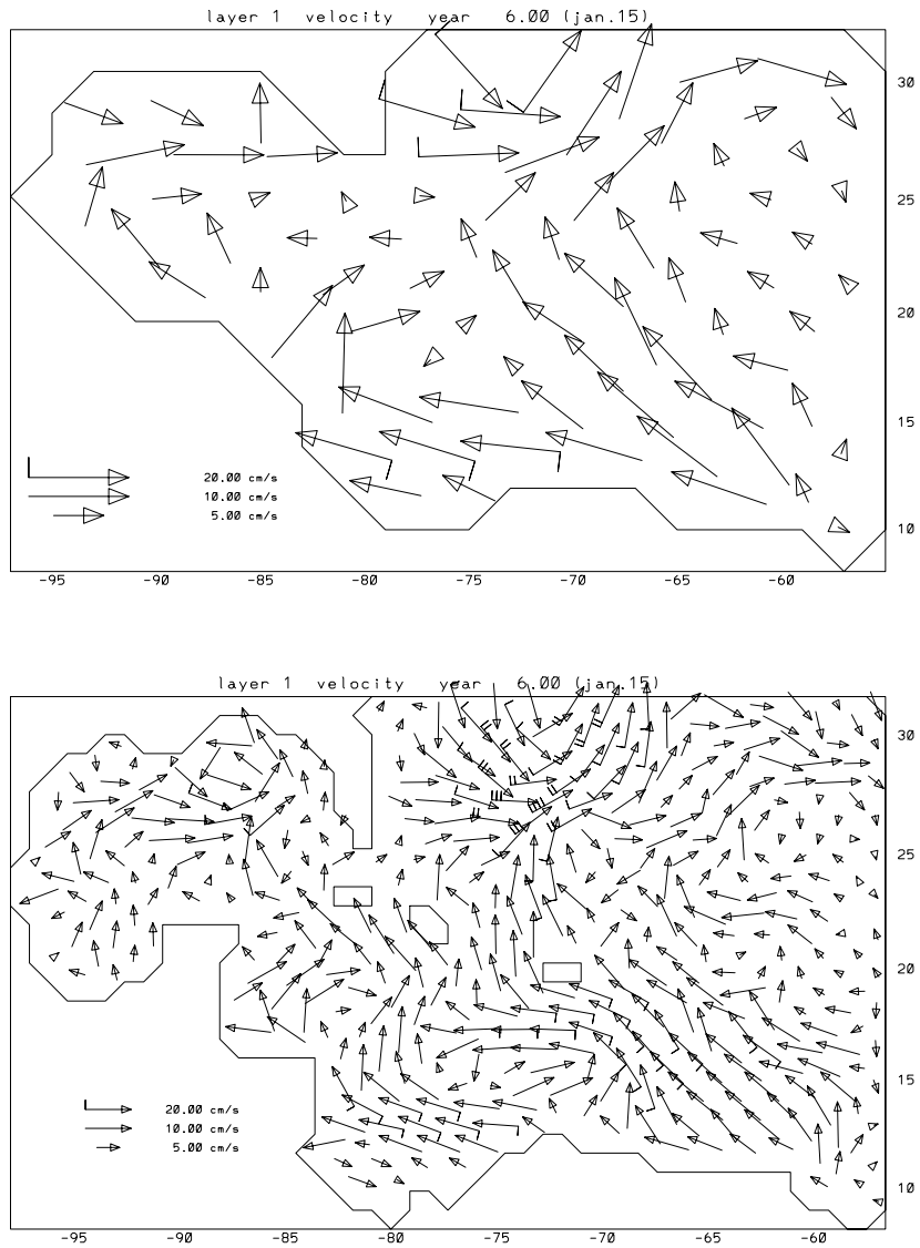
Figure 2: HYCOM surface velocities in the Carribeian Seas in the 2^\circ mesh North Atlantic control run (upper panel) and with finer resolution ( 1^\circ ) using boundary conditions from the control run.
