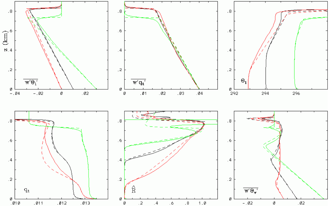
Figure 1. Mean vertical profiles from three sample large eddy simulations of quasi-steady cumulus-coupled boundary layers (red, black, and green lines) showing: liquid water potential temperature flux, total water flux, liquid water potential temperature, total water, R described in the text, and buoyancy flux. The solid lines represent a horizontal time average of the LES data and the dashed lines the predictions discussed in the text following from the entrainment constraints and given values for a limited set of physical inputs. The predictions provide a good representation of the LES data for all profiles.
