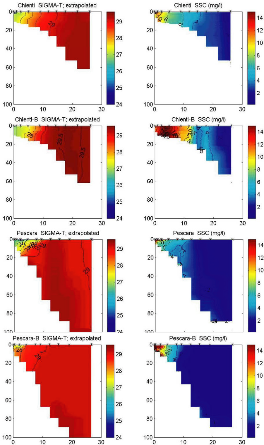
Fig.2 Density ( \sigma -t) and Suspended Sediment Concentration transects off Apennine Rivers. The top two panels are normal to shore, seaward of the Chienti River mouth, taken on Feb 14 and 19, 2003. Bottom two panels are off the Pescara River, on Feb 14 and 20, 2003. The 1 st and 3 rd panels follow a period of significant freshwater input, and the 2 nd and 4 th panels immediately follow a Bora wind event with diminishing wind speed. [Panels 2 and 4 show much higher suspended sediment concentrations extending farther offshore.]
