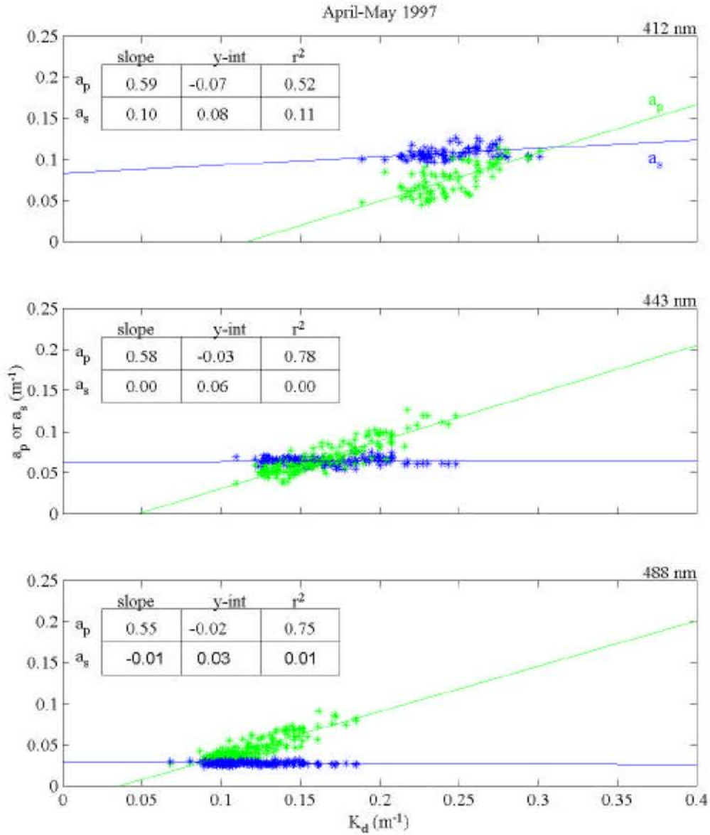
Figure 2. Relationships between diffuse attenuation for downwelling irradiance ( K_d ) and absorption coefficients for dissolved ( a_s ) and particulate ( a_p ) material at three wavelengths during April-May 1997. Data were collected and processed as described for Fig. 1. Linear regression results show strong dependence of K_d variations on a_p , with even less contribution of dissolved material than observed under conditions of greater stratification in late summer the previous year (Fig. 1).
