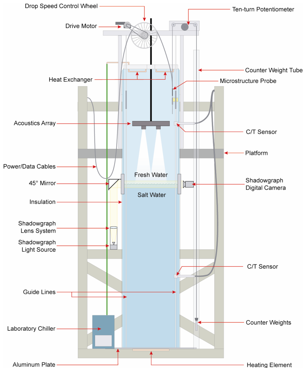
Figure 1. The experimental microstructure tank facility at Woods Hole Oceanographic Institution. The tank is 4.6 m (15 ft) high and 0.91m (3 ft) in diameter. Two opposing mid-depth windows, a bright white light source, focusing lenses, a 45° mirror, and a digital camera constitute the optical shadowgraph system. The high-frequency acoustics backscattering array can be positioned at any depth in the upper two meters of the tank. Temperature and conductivity sensors can be profiled through the tank and two CT sensors provide continuous monitoring of the top and bottom layer properties at two points. For the “diffusive convection” form of double diffusion a bottom layer of salty water is heated from below, while a top layer of fresh water is cooled by cooling coils suspended below insulating foam at the top. By introducing heating and cooling coils at other depths a stable temperature stratification suitable for salt finger or doubly-stable experiments can be obtained. By dropping grids through different temperature and salinity gradients turbulent temperature and salinity microstructure can be generated. By controlling the grid spacing and drop speed different characteristic turbulent length scales can be probed.
