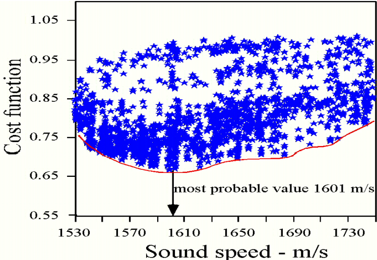
Figure 1: Cost function for surface sound speed of sediment.
