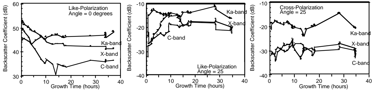
Figure 1. Observations of radar backscatter coefficients of the transition from open water to young sea ice when conditions are calm for C-, X-, and Ka-band frequencies, vertical and 25° angles of incidence, and like- and cross-polarizations.
