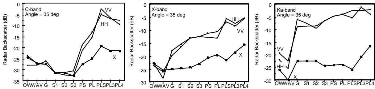
Figure 2. Observations of the microwave response of sea ice growth when waves are present include open water (OW), water with wave action (WAV), grease ice (G), slush ice (S), and pans of ice (P). Large pans are indicated with L, and the freezing of a pan surface with S. Numbers indicate an additional time increment in the decimal day of 0.05-0.1 days.
