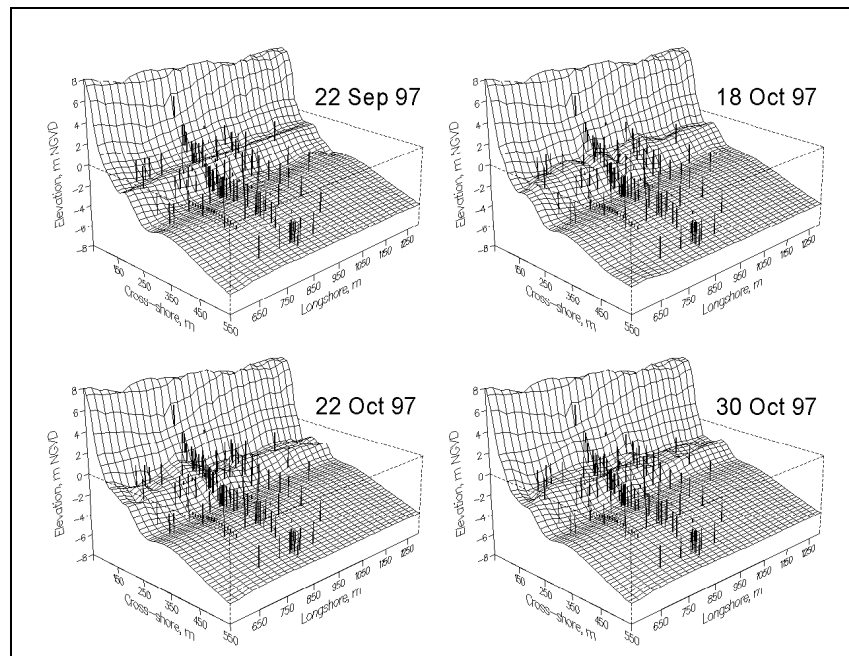
Figure 3. SandyDuck minigridded surveys including ones before and after the storm. Small vertical bars locate point sensors.
