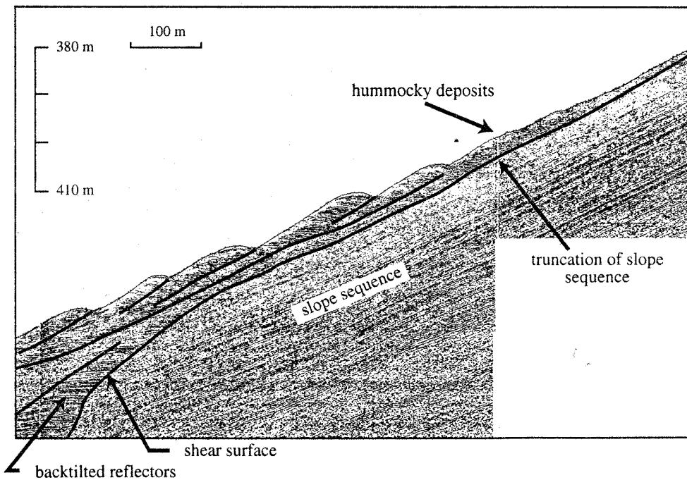
Figure 2. Huntex line showing upper portion of Humboldt Slide. Hummocky deposits bury the normal slope sequence. Shear surfaces separate sequences of reflectors. Vertical exaggeration 7X
