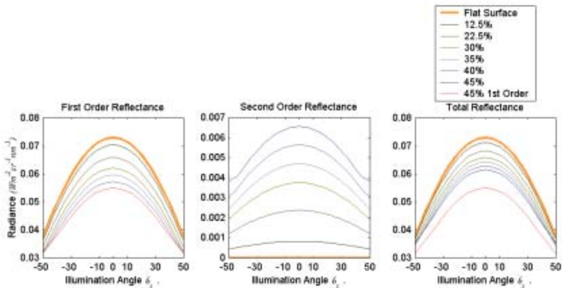
Figure 1. First and second order reflectances received by a nadir-viewing detector as wave amplitude changes and incidence angle varies.
