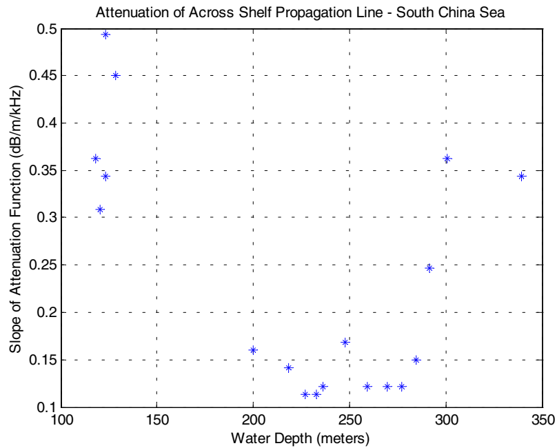
Figure 1. Attenuation rolloff for the frequency range of 1.6 to 4.0 kHz is plotted as a function of water depth for the across shelf propagation line. Note that the attenuation of the sediments is lowest for water depths in the range of 200 to 280 meters. Attenuation increases toward the ends of the across shelf propagation line indicating coarser grain sediments.
