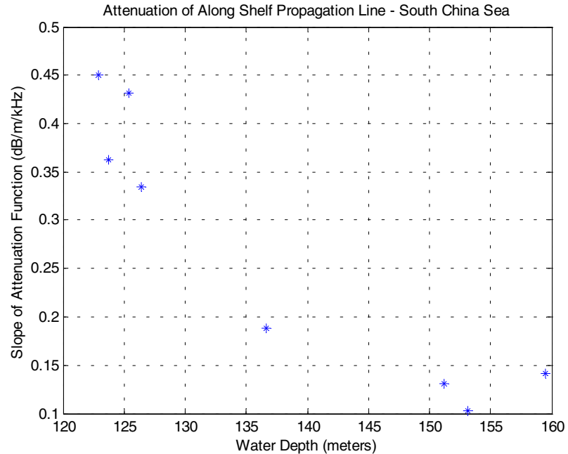
Figure 2. Attenuation rolloff for the frequency range of 1.6 to 4.0 kHz is plotted as a function of water depth for the along shelf propagation line. Note that the attenuation of the sediments is lowest for larger water depths suggesting that finer grain sediments occur in the deeper section of the line.
