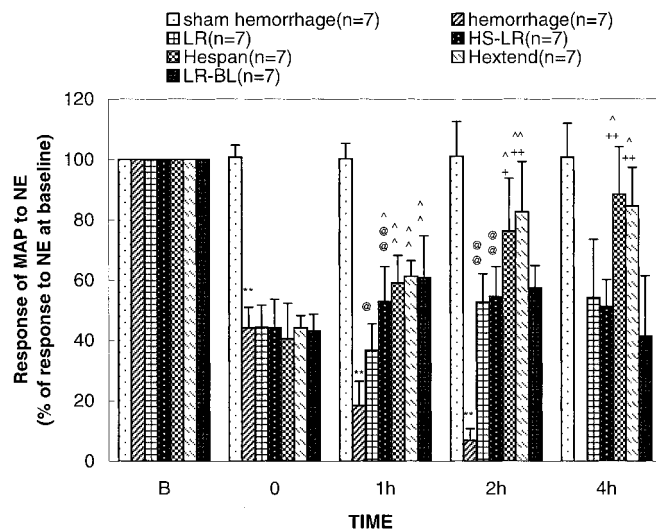
Fig. 3. Effects of crystalloid and colloid resuscitation on the pressor response of MAP to NE (3 \mu g/kg) after hemorrhagic shock in the rat. The increase in MAP after NE at baseline is considered a 100% response. B, baseline; Time 0, the end of the hypotensive period. n = 5 at 2 hours and n = 0 at 4 hours in the hemorrhage group; n = 7 at all other time points in each group. LR, lactated Ringer's solution infusion to a MAP of 70 mm Hg for 4 hours; HS-LR, 7.5% hypertonic saline infusion for 1 hour followed by lactated Ringer's solution to a MAP of 70 mm Hg for 3 hours; Hespan, Hespan infusion to a MAP of 70 mm Hg for 4 hours; Hextend, Hextend infusion to a MAP of 70 mm Hg for 4 hours; LR-BL, LR infusion to baseline MAP for 4 hours. No shed blood was reinfused in any group. Data expressed as mean \pm SD. At time 0, all hemorrhage groups are significantly lower than the sham hemorrhage group. ** p < 0.01 as compared with the sham hemorrhage group; @ p < 0.05, @@ p < 0.01 as compared with the hemorrhage group; ^ p < 0.05, ^^ p < 0.01 as compared with the LR group; + p < 0.05, ++ p < 0.01 as compared with the HS-LR group.
