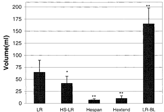
Fig. 1. Infusion volume of each fluid after hemorrhagic shock in rats. LR, lactated Ringer's solution infusion to a MAP of 70 mm Hg for 4 hours; HS-LR, 7.5% hypertonic saline infusion for 1 hour followed by lactated Ringer's solution to a MAP of 70 mm Hg, 41.4 \pm 14.9 mL in this group includes 2.16 \pm 0.47 mL of hypertonic saline; Hespan, Hespan infusion to a MAP of 70 mm Hg for 4 hours; Hextend, Hextend infusion to a MAP of 70 mm Hg for 4 hours; LR-BL, LR infusion to baseline MAP for 4 hours. Data expressed as mean \pm SD for seven rats per group. * p < 0.05 , ** p < 0.01 as compared with the LR group.
