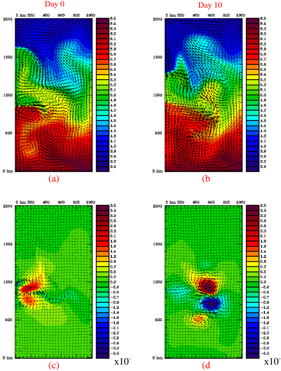
Figure 1: Idealized Double-Gyre Optimal Perturbations [Panels a and b show the surface temperature and velocity vectors of the double gyre basic state flow 10 days apart. Panels c and d show the surface velocity and sea level at initial and final times for the optimal perturbation that maximizes the growth of perturbation energy over the 10 day period.]
