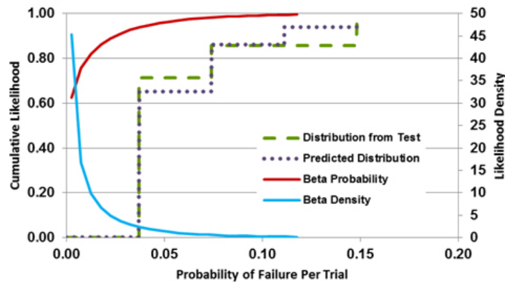
Figure 4.1: Likelihood for Example 1 (Section 3.1)
