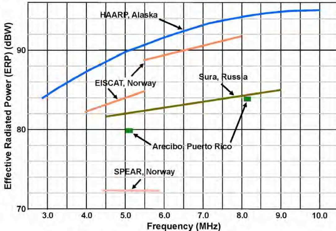
FIGURE 1.2 Effective radiated power versus frequency for current high-frequency heating facilities. The Arecibo facility is under construction and will come on line in 2014. NOTE: 1 GW is equal to 90 dBW. SOURCE: E. Kennedy, Naval Research Laboratory, "Heating facilities update: High-frequency Active Auroral Research Program (HAARP)," 4th Radio Frequency (RF) Ionospheric Interactions Workshop, Santa Fe, New Mexico, April 19-22, 1998.
