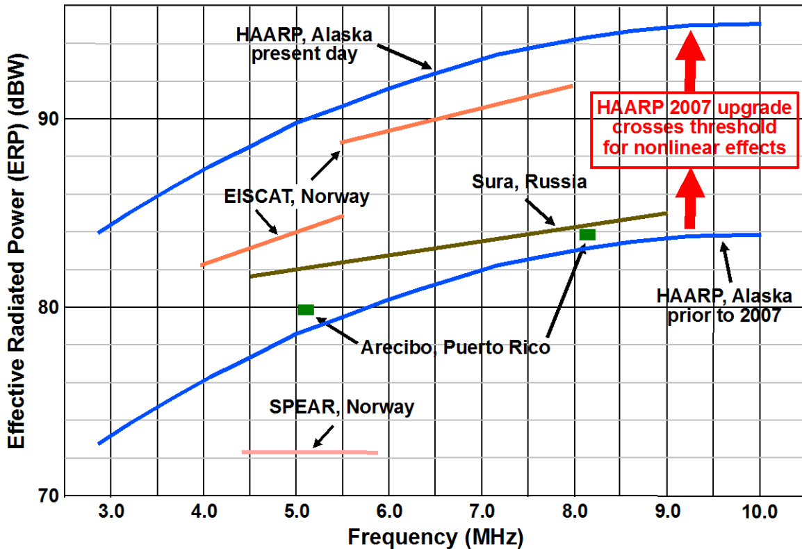
FIGURE S.4 Effective radiated power (ERP) versus frequency for high-frequency heating facilities. The performance of HAARP facility before the upgrade in 2007, which enabled the recent “unique and ground-breaking” results described in this report, is also indicated. The Arcibo facility is under construction and will come on line in 2014. NOTE: EISCAT, European Incoherent Scatter Scientific Association; SPEAR, Space Plasma Exploration by Active Radar. SOURCE: E. Kennedy, Naval Research Laboratory, “Heating Facilities Update: High-Frequency Active Auroral Research Program (HAARP),” 4th Radio Frequency (RF) Ionospheric Interactions Workshop, Santa Fe, New Mexico, April 19-22, 1998.
