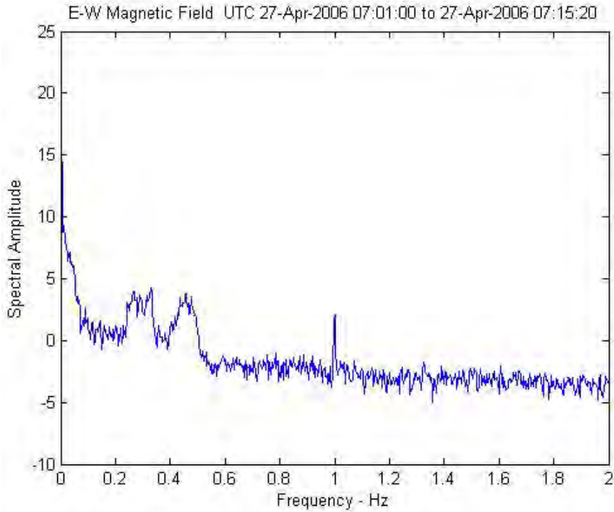
FIGURE 3.4 Natural excitation of the ionospheric Alfvén resonator at 0.25 and 0.5 Hz and artificial excitation by HAARP at 1 Hz. SOURCE: Courtesy of K. Papadopoulos, University of Maryland.
