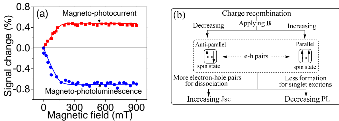
Fig. 7 (a) Magnetic field effect on photocurrent and photoluminescence. (b)Diagram to show the mechanism for magneto-optical effects in perovskites.
