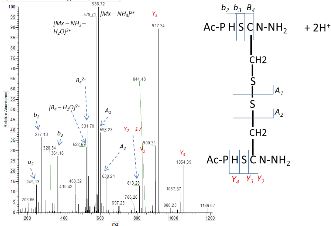
Figure 8. CID fragmentation of doubly-charged ion at 597.73 m/z (the second isotope to 597.23 m/z). Fragment ions B 4 , A 2 , Y 2 , Y 3 , and Y 4 containing S-S cross-linked peptides confirm disulfide bond formation between two thiols of cysteine.
