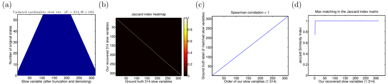
FIG. 4.5. Illustrative example CS-II. (a) The eigenvector-based slow variable cardinality after truncating and bin denoising. The Theta score \Theta is the smoothness measure of the bin cardinalities, defined in (4.5). (b) The heatmap of the pairwise Jaccard similarity matrix given by (4.4). (c) The correlation between the ordering of the ground truth slow variable and the eigenvector recovered slow variable. (d) The Jaccard index of the pairwise matched bins (from the maximum matching).
