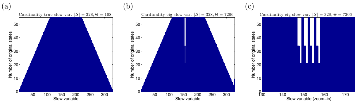
FIG. 4.4. Illustrative example CS-II. (a) The ground truth slow variable cardinality. (b) The eigenvector-based slow variable cardinality. \Theta captures the smoothness of the bin cardinalities, as introduced in (4.5). (c) Plot of the cardinalities of a subset of bins, showing the erroneous bin assignments in the eigenvector-based partition. This is a zoomed-in version of panel (b).
