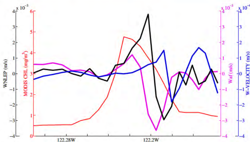
Figure 5. The model vertical velocity W (blue), the nonlinear Ekman pumping W_{nlep} (black), and the vertical velocity due to frontogenesis W_{af} (magenta) are plotted along the same section as in Figure 4a. All three velocities are averaged over a period of 48 h centered on 15 August 00Z and over the top 15 m depth.
