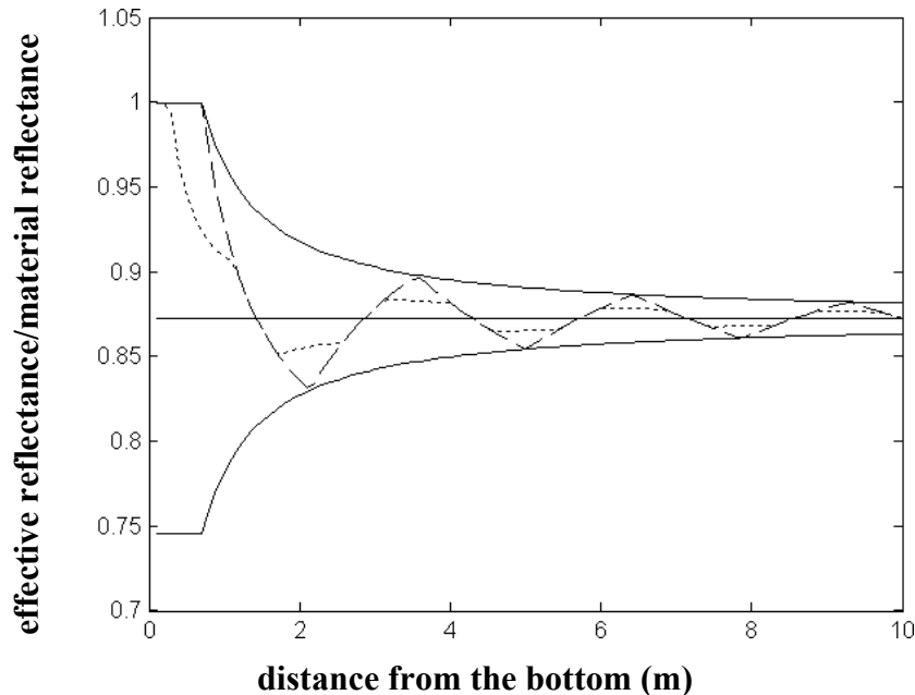
Fig.2. Example of near field effective reflection relative to the material reflection. [graph: Near field effective reflection relative to the material reflection as a function of distance from the bottom for a saw-tooth bottom with an amplitude of 0.025 m and a wavelength of 0.25 m. The detector has a 5 degree half angle field of view. The upper and lower curves are the maximum and minimum reflectances that can be detected. The far field reflectance relative to the near material reflectance is 0.75. This is always the relative reflectance if the detector is located directly above the interface of two facets. Maximum variability is obtained when the detector is located directly above the center of a facet (dashed line). The relative reflectance is truncated when the detector is neither directly above the edge or center of a facet. The dotted line is for a detector that is directly above a point 0.2 wavelengths from the edge of a facet.]
