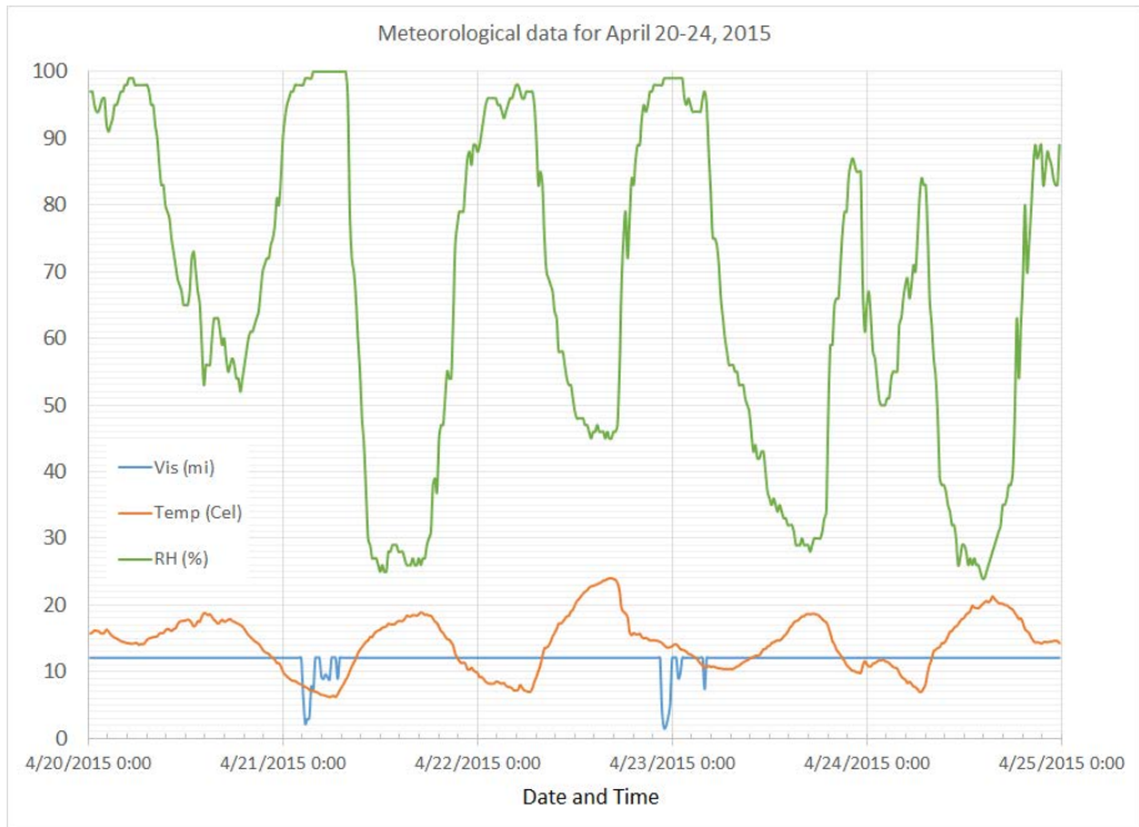
Fig. 17 Measured visibility (miles), air temperature (°C), and relative humidity (%), for the week of April 20–24, 2105
