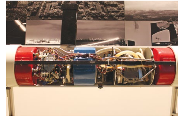
The proof-of-concept fuel cell for an autonomous underwater vehicle (AUV) was developed through a collaboration between Laboratory researchers and students in an MIT mechanical engineering course. The current project is to design the fuel cell to fit in an actual AUV.
