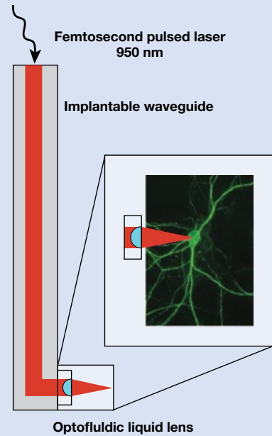
This conceptual schematic shows a novel liquid-lens-coupled brain probe used for mapping neural activity at single-cell resolution.
