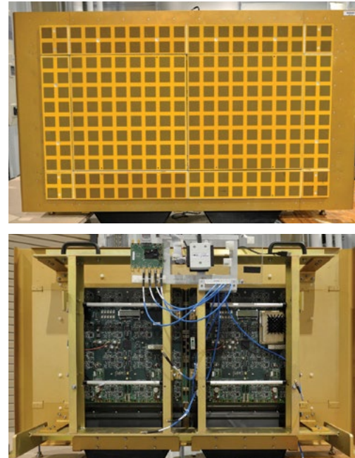
These photos show the front (top) and back (bottom) views of the 128-element dual-polarization Multifunction Phased Array Radar (MPAR). The Laboratory is currently building a mobile demonstration radar with a 640-element array that will be deployed for field testing.
