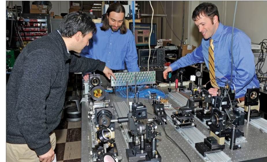
Juan Montoya, Andrew Benedick, and Scot Shaw use prototype technology to demonstrate a new optical phased array beam-combining approach developed at Lincoln Laboratory with support from the Defense Advanced Research Projects Agency (DARPA).
