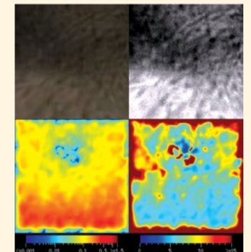
The Digital Vision Sensor (DVS) was programmed to compute optical flow, i.e., the apparent motion of brightness in a scene at high frame rates. This image shows the optical flow processing (clockwise from upper left) for a simulated 3D scene: rendered scene image, simulated DVS image, computed optical flow magnitude (pixels/frame), and derived scene depth (meters).
