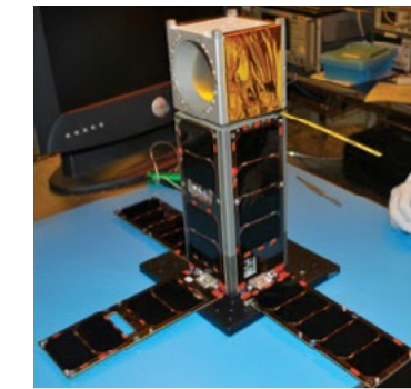
An Orbital Sciences Cygnus cargo spacecraft delivered the Micro-sized Microwave Atmospheric Satellite (MicroMAS) CubeSat, shown above with its solar arrays opened, to the International Space Station (ISS) on 13 July 2014 as part of the Orb-2 cargo resupply mission launched from the Mid-Atlantic Regional Spaceport in Virginia. The NanoRocks CubeSat Deployer, shown in the left photo, will be used to put MicroMAS into position for space-based terrestrial weather sensing.
