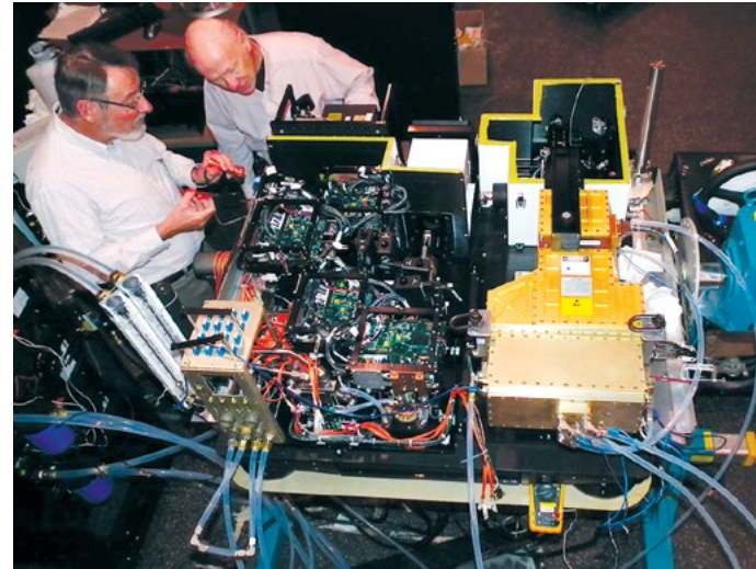
The MACHETE ladar sensor is successfully integrated onto a DHC-8 aircraft.
