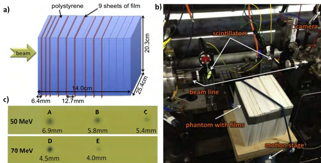
FIG. 1. Schematics (a) and a photograph (b) of the experimental setup for measurements of 50 and 70 MeV VHEE beams with Gafchromic EBT2 films (c) at the NLCTA beam line of SLAC National Accelerator Laboratory. Films were sandwiched in a 14-cm deep polystyrene phantom and irradiated at five locations with pencil beams of FWHMs ranging from 4.0 to 6.9 mm as measured on the film at 0.64 cm depth (c).
