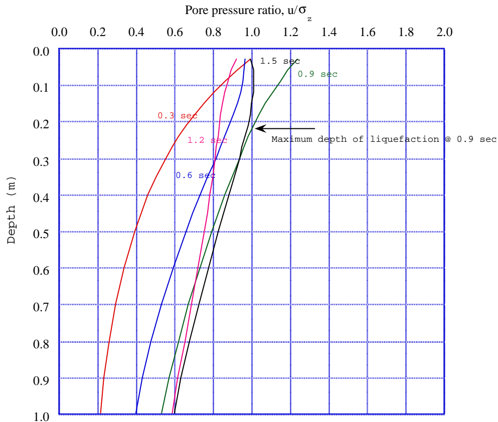
Figure 3. Drained excess pore pressure distribution with depth [maximum excess pore pressures does not coincide with the crest of the wave]
