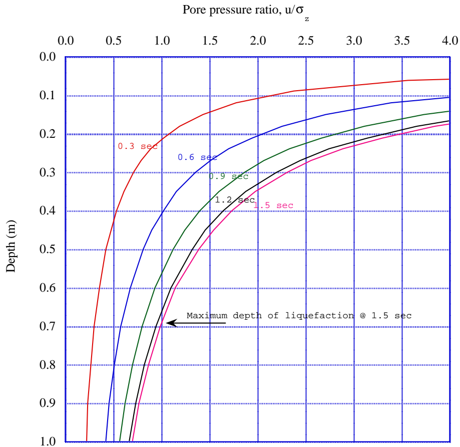
Figure 2. Undrained excess pore pressure distribution with depth [maximum excess pore pressures coincide with the crest of the wave]
