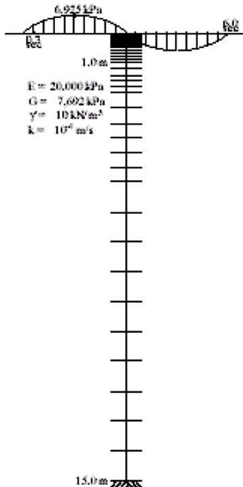
Figure 1. 1-D Finite element discretization of 15 m seabed below sinusoidal seabed pressure
