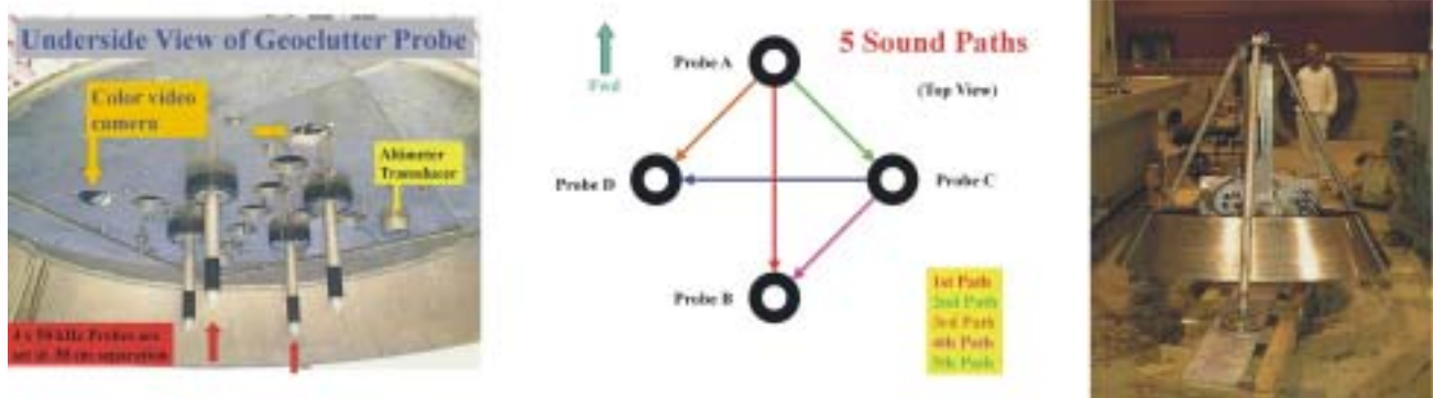
Fig 2. Underside view of ISSAP showing orientation of probes (left), diagram showing 5 paths used for sound speed and attenuation measurement (middle) and photo of tripod and probe assembly (right).
