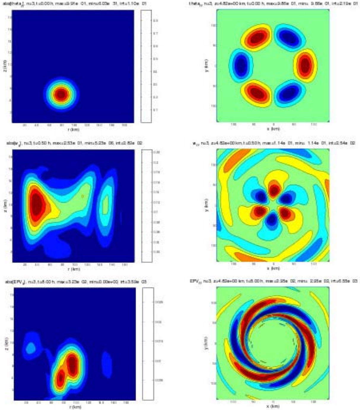
Figure 1. Linear evolution of a purely thermal perturbation near the core of a weak, baroclinic, tropical storm-like vortex. The first two plots show r - z and x - y cross-sections of the initial disturbance in \theta . The next two show cross-sections depict vertical velocity at t = 30 min, showing gravity wave propagation. The last two cross-sections show perturbation PV at t = 8 h, showing interaction with the mean vortex and axisymmetrization.
