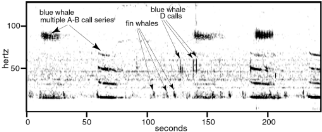
Figure 2. Sonobuoy acoustic data from the SCORE area showing blue and fin whale calls.
