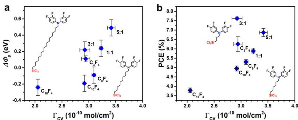
Figure 8. (a) Work functions of ITO/SAM/SHSAMs and (b) power conversion efficiencies (PCEs) of OPVs fabricated from ITO/SAMs/SHSAMs as a function of corresponding cyclic voltammetry determined packing densities. In general, higher IFL packing densities correlate with higher work functions and OPV metrics.
