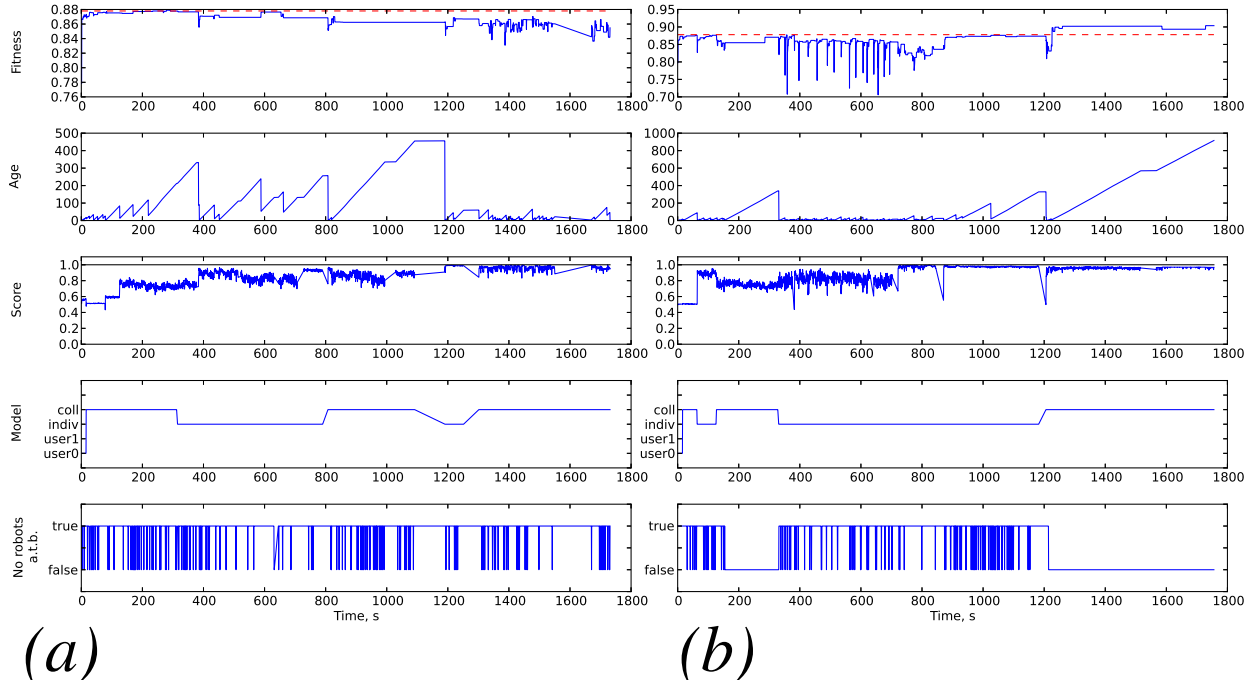
Figure 5: Time series for some parameters of the server over the course of typical allied simulations: (a) an unsuccessful simulation and (b) a successful simulation. The three topmost graphs represent the unscaled fitness f_u , age and the coordinated score \sigma of the current best controller in the evolutionary population (computed using the product f_u\sigma ). The red dotted line in the fitness graph (top) shows a rough estimate of the maximal value of f_u which the robot not going around the barrier can have (0.88). The fourth graph from the top shows how the way in which the server modeled users changed over the course of the simulation: “coll”, “u0” and “u1” indicate the usage of the collective user model and the individual models of the first and the second user, correspondingly; “indiv” corresponds to the two users being modeled separately. See the Coordinated Score Generation section for details. The graph at the bottom gives the logical value “No robots above the barrier”: false if there are any controllers in the current population which make robot travel beyond the barrier (i.e., have Y \geq Y_b at some point of the behavior simulation) and true otherwise.
