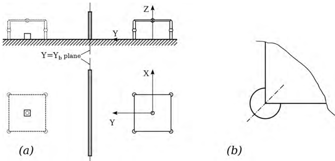
Figure 3: Test problem. (a) Side and top views of the robot and its environment at the beginning of the simulation. The small square to the left denotes the light source; spheres on the robot's body are light sensors. The target position that the robot should reach is depicted with dotted lines. Y_b denotes the Y coordinate of the barrier. (b) Joint between the robot's main body (square plate) and a limb, top view. The dotted line denotes the axis of rotation. The angle of the limb's rotation relative to its default position (as in (a)) can take values in [-45^\circ, 45^\circ] . A video of the robot with a successfully evolved controller can be viewed at http://youtu.be/ByDfAcDBsHI .
