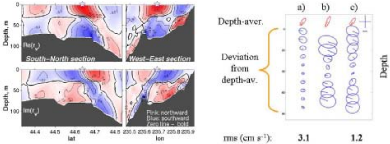
Figure 1. Left: The representer r_s , showing the zone of influence of the surface alongshore velocity measurement on the modeled M_2 tidal alongshore current off central Oregon. The star shows the observation location. Right: Tidal ellipses at the ADCP location: a) model only solution forced by depth-averaged currents, b) ADCP data, c) inverse solution. Numbers under the plot show the rms difference of the solutions and the ADCP data.
