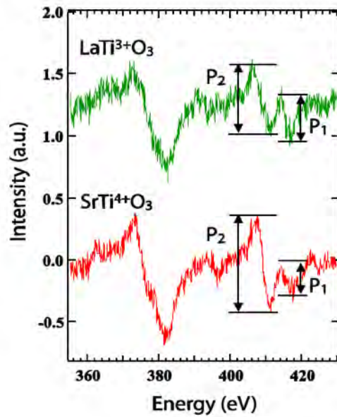
Figure 5. XPS excited Auger spectra which allows to determine the charge states of Ti. Specifically, the ratio of P1/P2 is sensitive to the valence state of Ti which can be used to distinguish between Ti 3+ and Ti 4+ .
