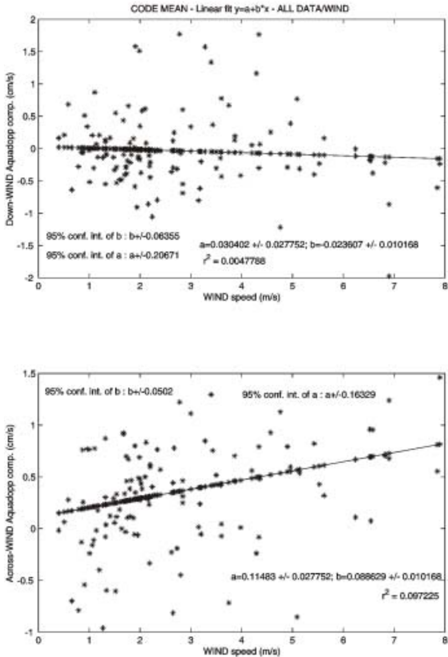
Fig. 2. Mean down-wind (top) and cross-wind (bottom; positive to the right) slip speeds versus wind speed measured for the CODE drifter in Monterey Bay (5-12 December 2000). Mean slips were obtained by averaging the relative flows measured by the acoustic velocimeters at the top and at the bottom of the drifter.
