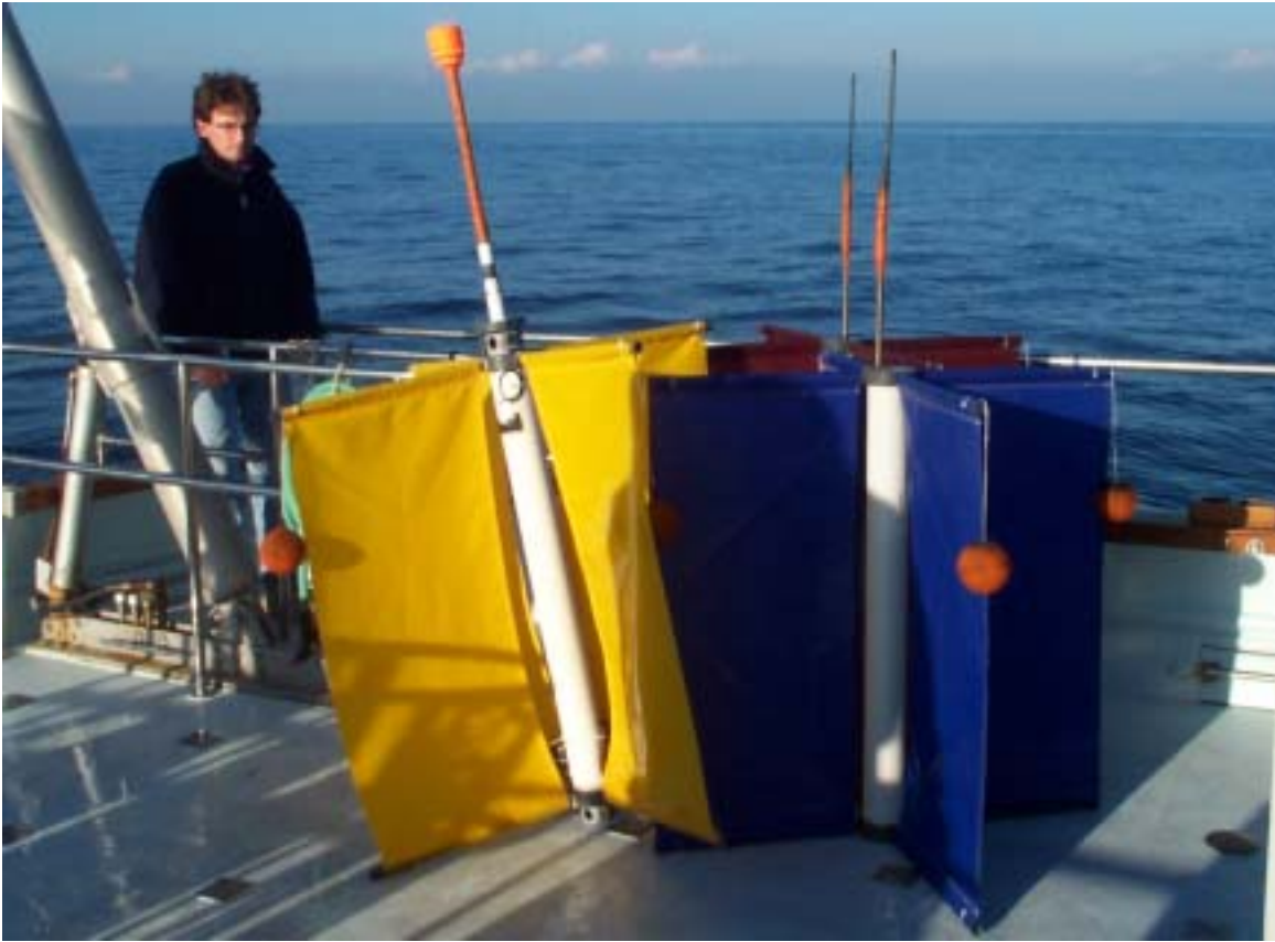
Fig. 1. CODE drifters ready to be deployed in Monterey Bay in December 2000: Two standard designs with Argos antenna are shown to the right (brown and blue); the drifter equipped with two acoustic velocimeters and GPS antenna is shown to the left (yellow).
