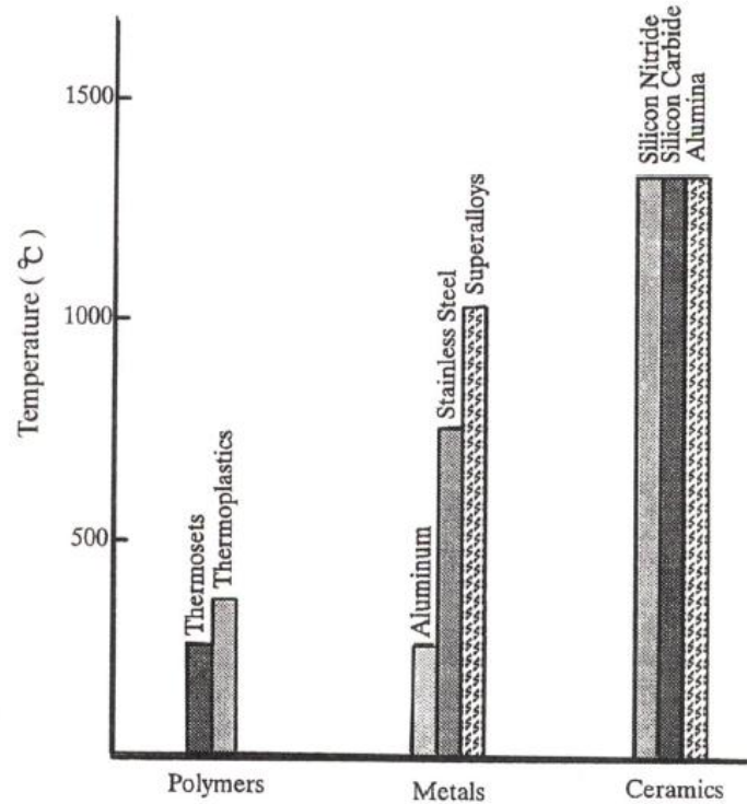
Figure 2: Service temperature limits of various classes of materials; Reproduced with kind permission from Springer Science & Business Media B.V. [1] pg. 5, Chapter 1: Introduction, Figure 1.3. Copyright c 2003 by Kluwer Academic Publishers. All rights reserved. No part of this work may be reproduced, stored in a retrieval system, or transmitted in any form or by any means, electronic, mechanical, photocopying, microfilming, recording or otherwise, without the written permission from the Publisher, with the exception of any material supplied specifically for the purpose of being entered and executed on a computer system, for exclusive use by the purchaser of the work.
