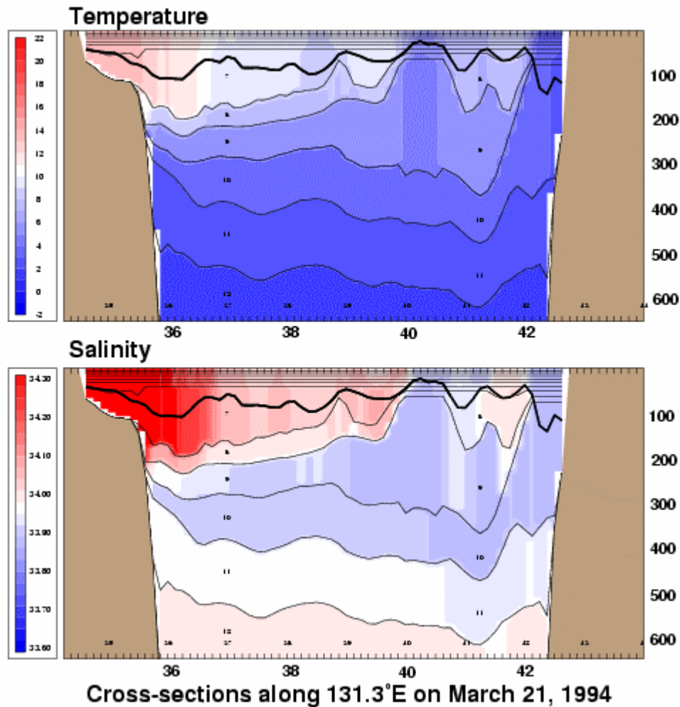
Figure 1. Simulated cross-sections of temperature and salinity along 131.3°E from a 1/16°15-layer HYCOM simulation in the JES. The Tsushima Strait is to the left, Vladivostok is to the right. The simulation was forced with 6 hourly 10m winds and thermal fluxes from the ECMWF reanalysis product, as well as throughflow through the straits. These snapshots, for March 21, 1994, show a deep mixed layer near Vladivostok and the associated cold water extending from the surface to intermediate depth (300-400m). The bottom panel shows the relatively low salinity ESIW (blue) forming at the surface near Vladivostok, sinking to intermediate depth, and advecting southward towards the Ulleung Basin.
