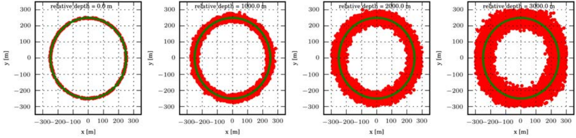
(b) Approximate posterior distribution over state given 2D pseudo range and depth observations.
