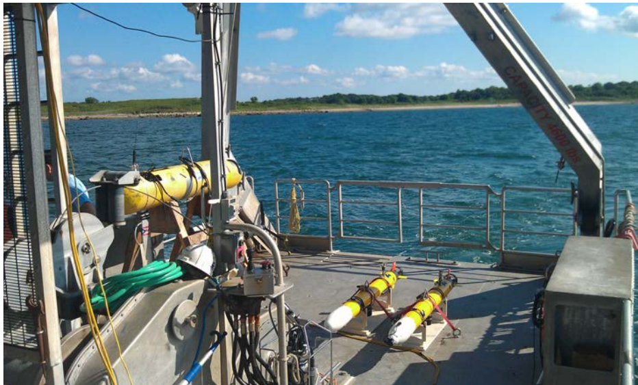
Figure 1.4 AUVs onboard the R/V Tioga in Buzzard’s Bay, MA. The two adjacent AUVs on deck were used for experimental validation throughout this thesis.
