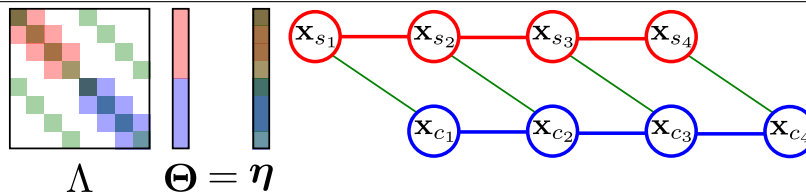
Figure 2.2 Joint pose-graph (MRF) over server, \mathbf{x}_{s_i} , and client, \mathbf{x}_{c_j} , poses where \Theta is a vector including server and client poses, \Lambda is the information matrix, and \eta is the information vector. Green lines illustrate edges generated by relative range observations between server TOL poses and client TOA poses. In order to construct the full pose-graph, the client must have access to the server’s local information (shown in red).
