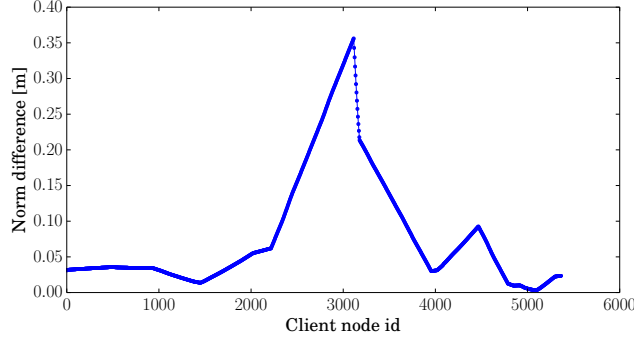
Figure 2.17 Difference in estimated pose between the DEIF algorithm and the nonlinear least-squares iSAM during Experiment F. The mean and maximum differences are 0.079 m and 0.35 m, respectively.
