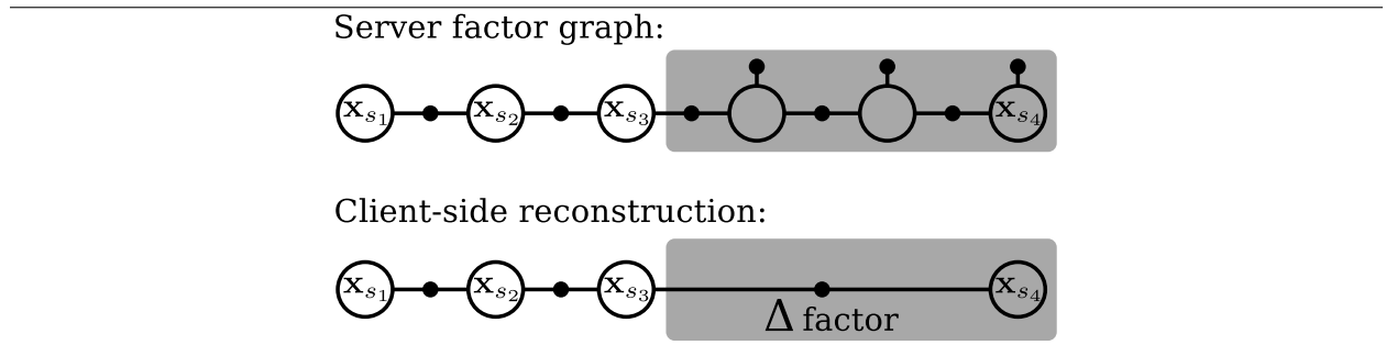
Figure 2.16 Server factor graph example. The above factor graph shows the full server factor graph. Shaded nodes and edges indicate constraints occurring between the previous and current TOL. The lower graph illustrates the reconstructed client-side factor graph. The shaded delta state factor induces an equivalent factor potential as the original server-side factors.
