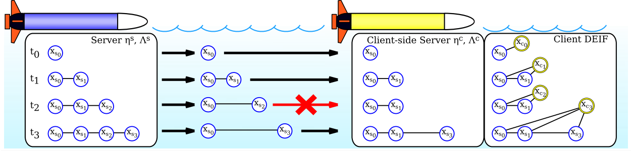
Figure 2.1 Origin state method algorithm overview: the server (blue) fuses its local observations and adds delayed-state poses at each time-of-launch (TOL) (the blue circles). The server uses our novel origin state method to incrementally broadcast its pose-graph in a fault-tolerant way. At the time-of-arrival (TOA) of each received origin state packet, the client (yellow) reconstructs the server pose-graph and updates its estimator to fuse all new information. In this example, although the client misses the server transmission at t_2 , the client still reconstructs the server pose-graph after receiving the origin state packet at t_3 , which encapsulates all server information accumulated between t_1 and t_3 .
