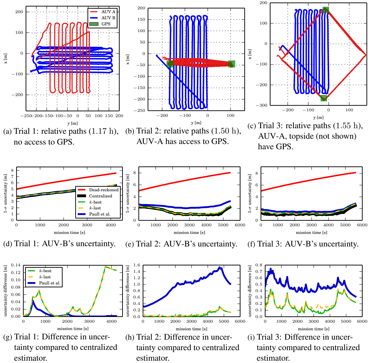
Figure 3.6 Summary of field trials and performance comparison. (a–c) shows each vehicle trajectory. (d–f) plots the smoothed uncertainty in each AUV-B pose computed as the fourth root of the determinant of the pose marginal covariance. AUV-A access to GPS is indicated by green boxes.
