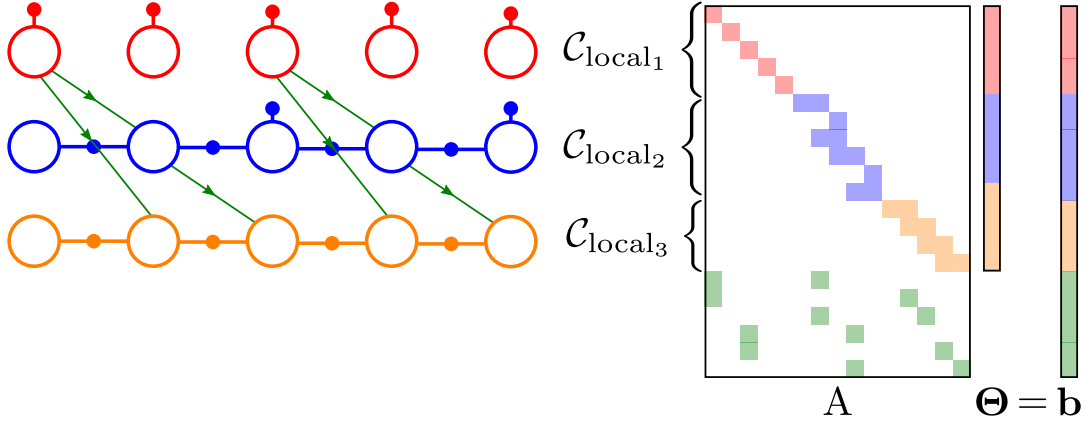
Figure 3.1 Example cooperative localization factor graph—empty circles represent variable pose nodes, solid dots are odometry and prior factors, and arrows illustrate range-only factors and the direction of communication. In this example, red represents a topside ship with access only to GPS, while blue and orange represent AUVs. Take note that the dashed blue factors represent a new set of approximate factors distinct from the original in (a).
