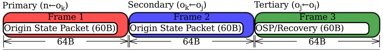
Figure 2.10 Acoustic message composition. Each PSK Rate 1 and Rate 2 Micro-modem message contains three 64-byte frames. We use the first two frames to hold two origin state packets and the third frame is reserved for recovery packets, or an additional origin state packet if no recovery has been requested.
