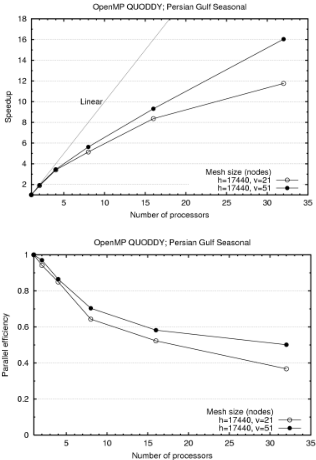
Figure 2. Parallel (a) speed-up and (b) efficiency of the Open-MP implementation in QUODDY for seasonal circulation simulations. Near-linear speed-up up to 8 processors for a 17440 node problem. Efficiency linearly decreases to 60-70% for up to 8 processors with continued slight decreases using more processors. Greater numbers of vertical nodes increase efficiency by 10%. All simulations are performed on the SUN Enterprise 10,000.
