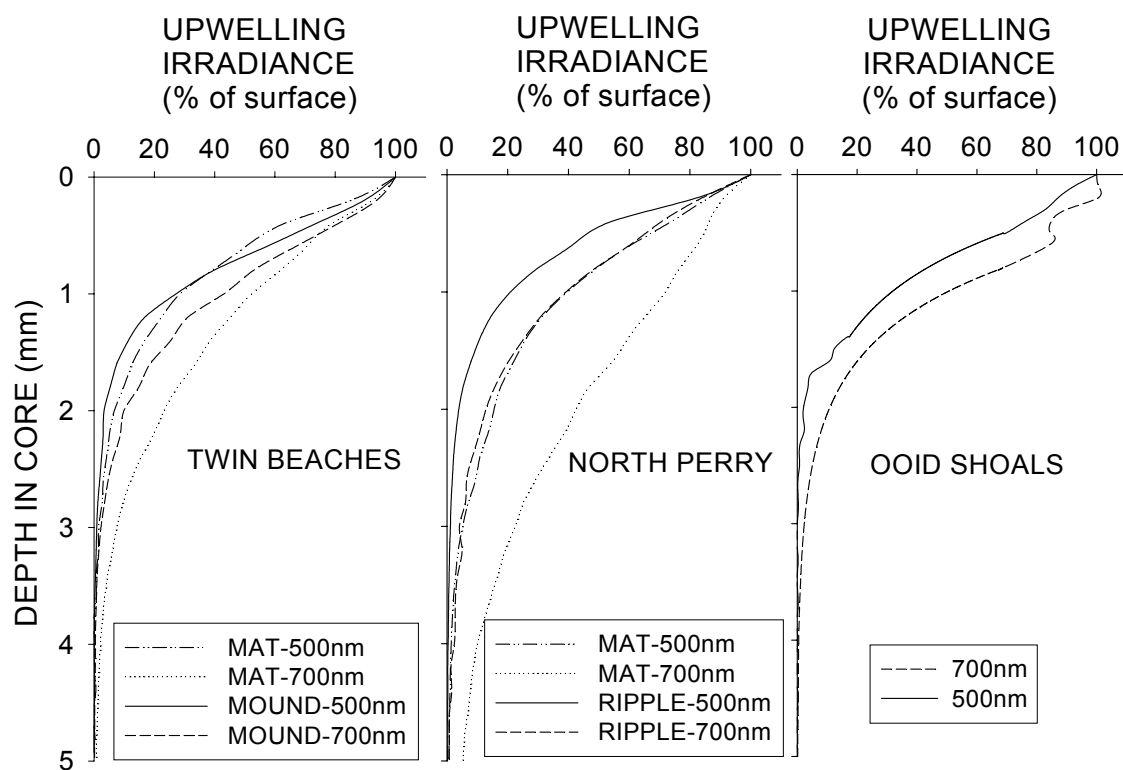
Figure 1. Plot of light penetration depth relative to levels measured at the sediment surface for all three study sites in April 2001 using the fiber-optic microprobes. Each plotted curve is an average of 3-6 measured profiles from a single core measured at 0.1 mm intervals downcore. In both sites where mats are found (North Perry and Twin Beaches), the depth of light penetration was greater than bare sands at the same wavelength. The bare sediment samples were collected from Callianassa mounds at Twin Beaches, and migrating ripples at North Perry and Ooid Shoals.
