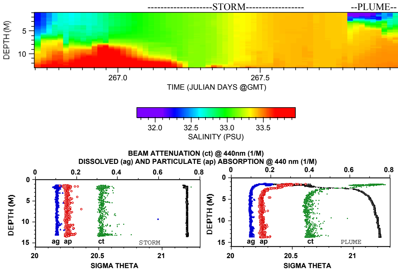
Figure 1. A 31 hour time series of fine scale salinity structure quantified by ORCAS in the Gulf of Mexico 2 km off Pensacola, Fl. During the first 6 hours winds were calm and the system had a strong halocline with at 8-12 m. As winds increased over the next 12 hours to speeds in excess of 25 knots, the halocline deepened until the entire water column was isohaline (well mixed). The water column remained isohaline until 26 hours into the record, at which point surface water salinity dropped 3 PSU re-establishing a halocline that deepened over time. This transition took less than 15 minutes as one might expect when the frontal edge of a buoyant surface plume is advected into the profiler's area. As indicated in the lower panels, optical properties (dissolved absorption, particulate absorption and beam attenuation) more than doubled inside the plume relative to the storm. Optical structure was measured by our ship-deployed high resolution profiler using the dual ac-9 technique (Twardowski, et al, 1999)
