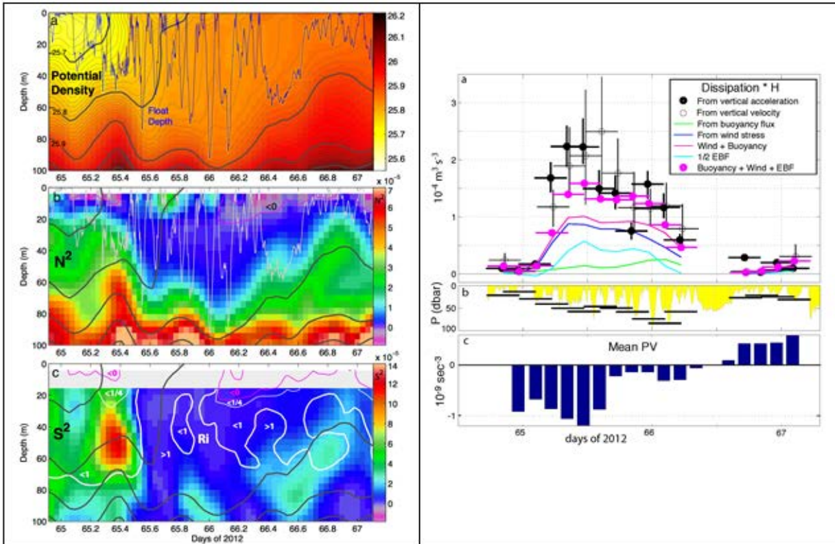
Figure 1. Evolution of vertical structure within the North Wall of the Gulf Stream during the 2012 winter experiment. Left: a) potential density (contoured and colored) and float depth (blue line). b) Vertical density stratification expressed as buoyancy frequency squared (colored). Boundary of unstable regions are indicated by the magenta lines. Float trajectory is repeated from panel a. c) Vertical shear squared (colors) and Richardson number = buoyancy frequency squared over shear squared (white contours). Selected density contours as in panel a. Right: a) Time series of boundary layer integrated dissipation estimated from float acceleration spectrum (black solid symbol) and from float vertical kinetic energy (black opensymbol). Expected dissipation from various forcings: buoyancy flux (green line), wind stress (blue line), their sum (red line), Ekman Buoyancy flux (cyan line) and the sum of all forcings (magenta symbol). b) Float depth during Lagrangian drifts (yellow filled) and boundary layer depth for each time window (heavy black) estimated as twice the mean float depth. c) Mean potential vorticity in the boundary layer.
