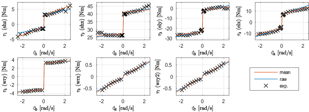
Figure 52. Joint friction diagrams from constant velocity experiments
