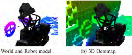
Fig. 4: World model of a valve scenario with robot model and the 3D Octomap for planning.
