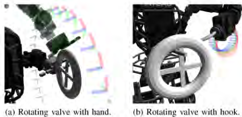
Fig. 6: Circular path plan to turn a valve 360 degrees. In (a) the hand rotates around changing its orientation, while in (b) the hook rotates around keeping its orientation. Interpolated poses are shown for the last joint of the arm.
