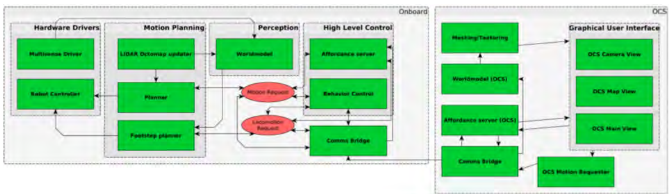
Figure 9. Software Architecture
